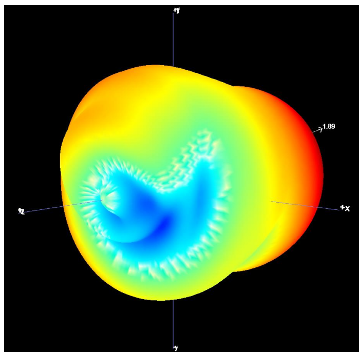
B1.3 3D Pattern for 930MHz
