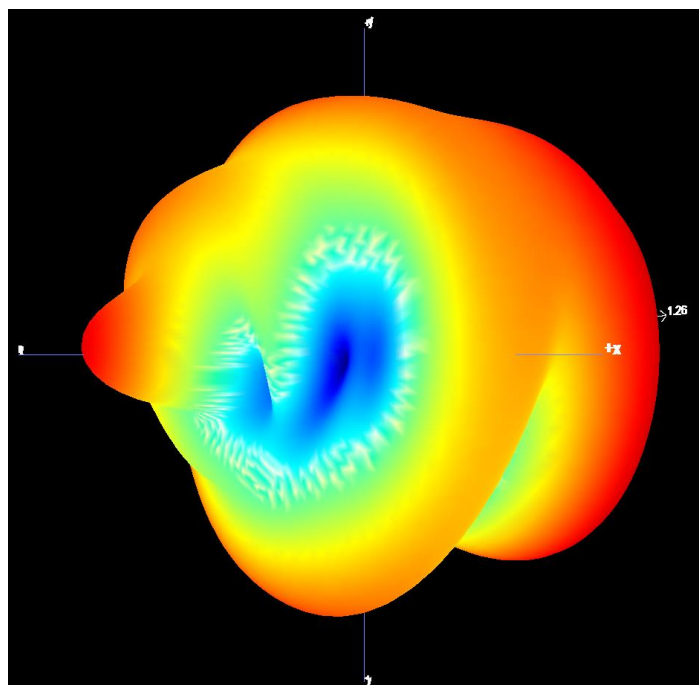
B1.1 3D Pattern for 890MHz
