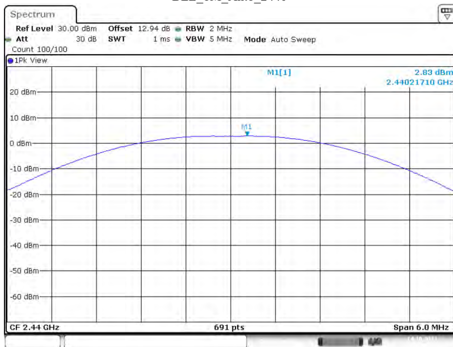
BLE_1M_Ant1_2440
