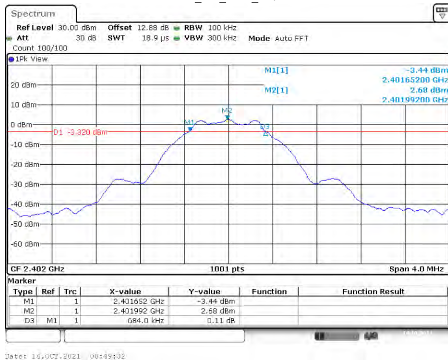
BLE_1M_Ant1_2402
