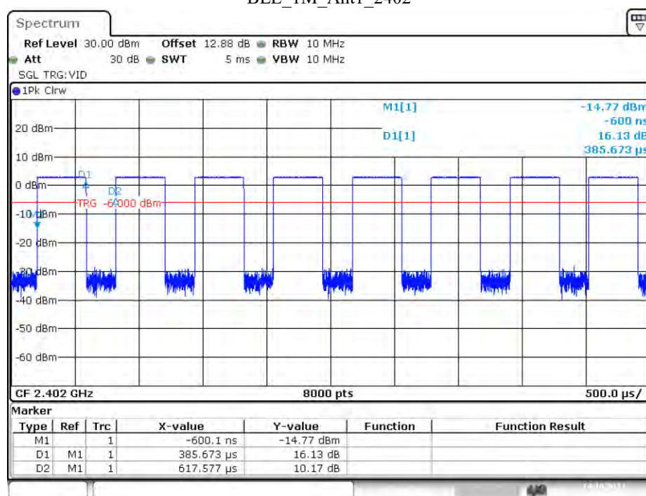
BLE_1M_Ant1_2402
