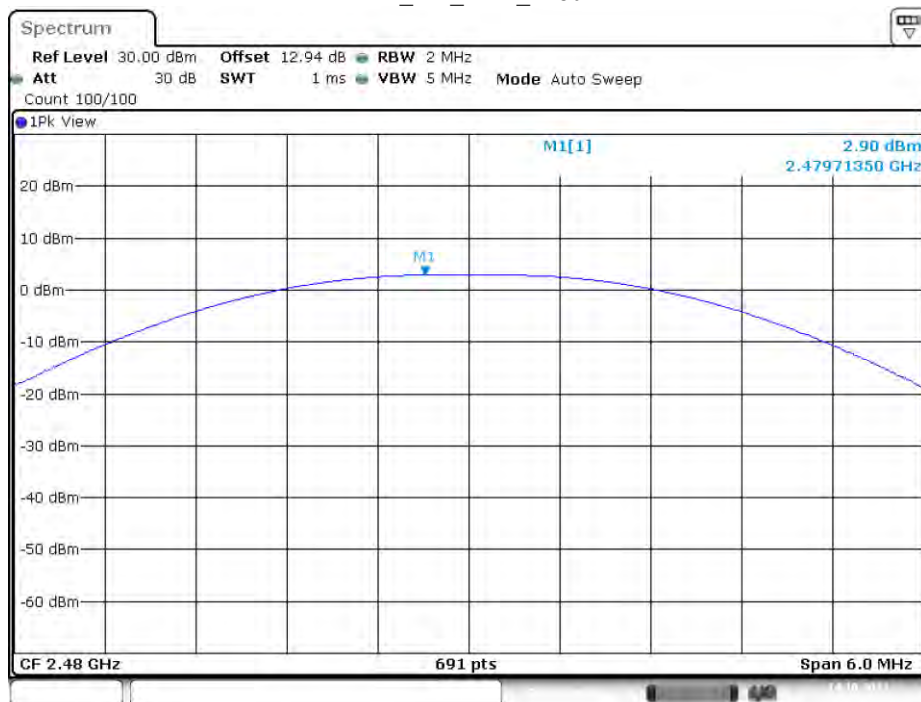
BLE_1M_Ant1_2480
