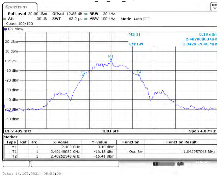
BLE_1M_Ant1_2402
