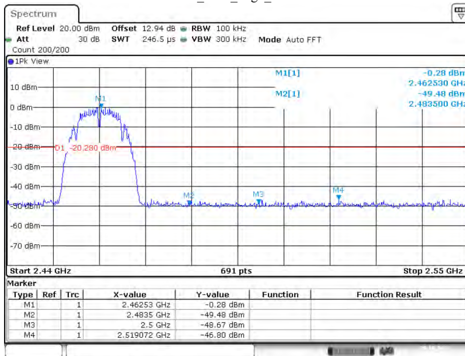
11B_Ant1_High_2462
