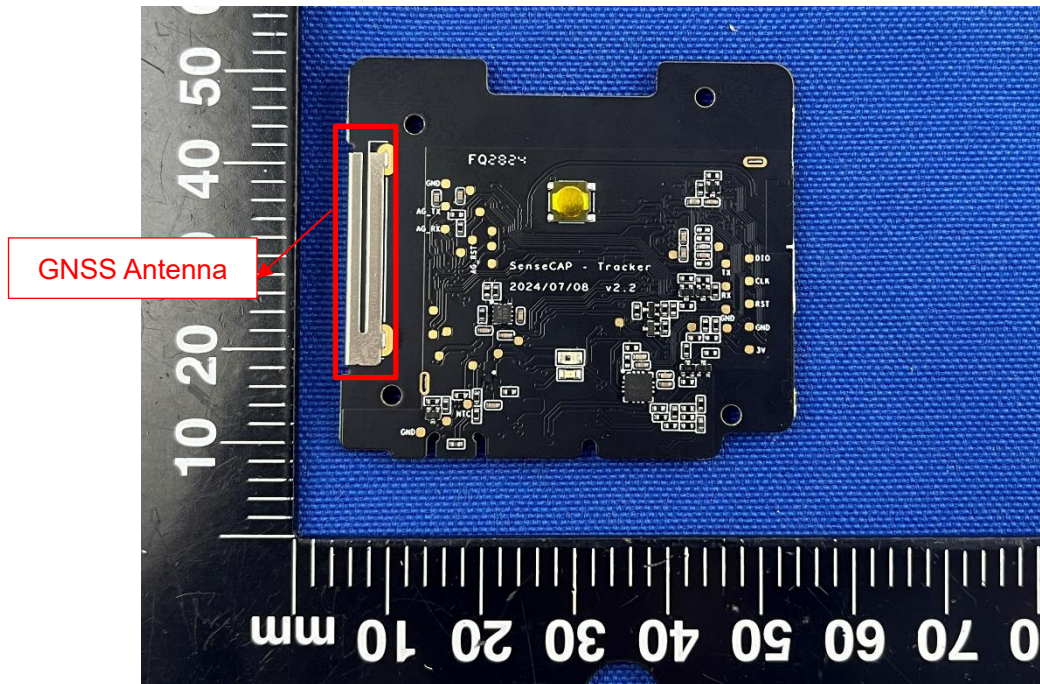
MAIN BOARD REAR VIEW (WITH SHIELDING)
