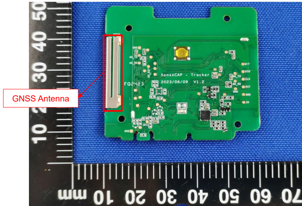
MAIN BOARD REAR VIEW (WITH SHIELDING)
