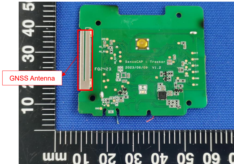
MAIN BOARD REAR VIEW (WITH SHIELDING)
