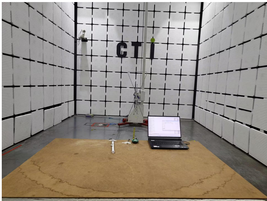
Radiated spurious emission Test Setup-1(Below 1GHz)-3
