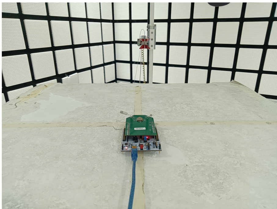
Radiated spurious emission Test Setup-2(Above 1GHz)-3
