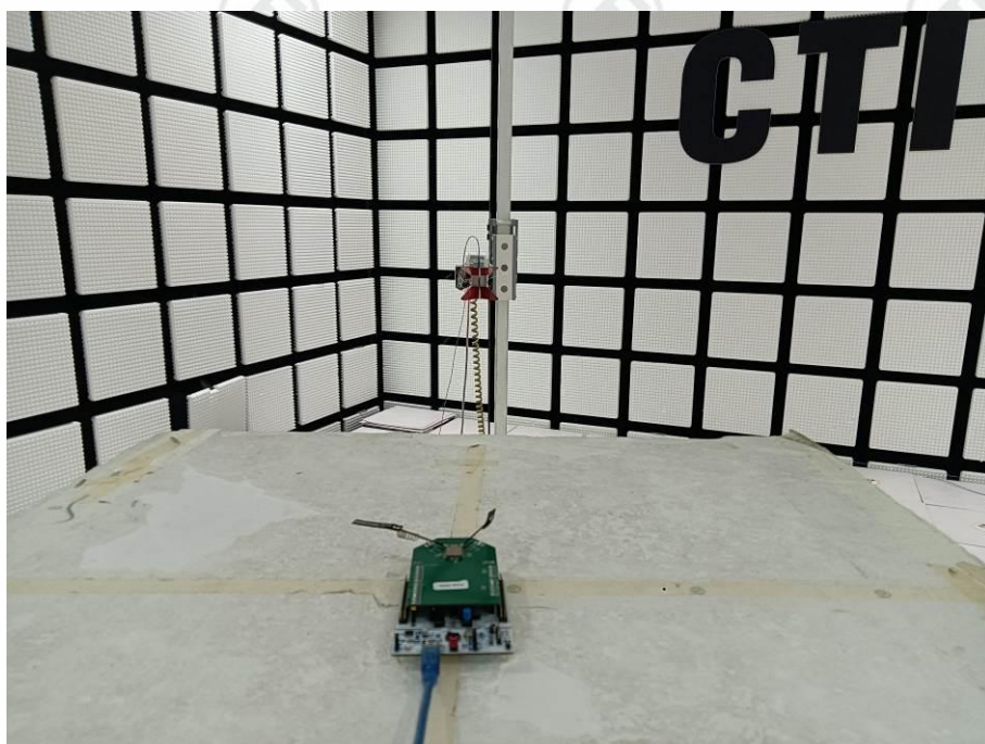
Radiated spurious emission Test Setup-2(Above 1GHz)-1
