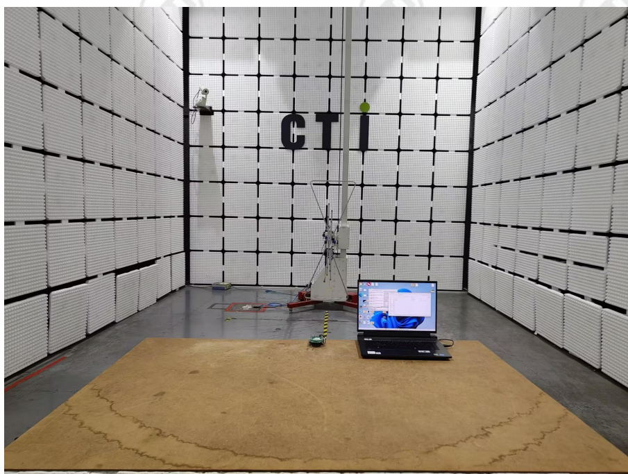
Radiated spurious emission Test Setup-1(Below 1GHz)-2
