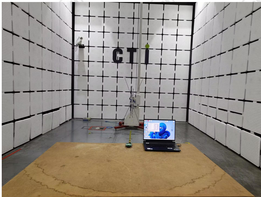
Radiated spurious emission Test Setup-1(Below 1GHz)-1
