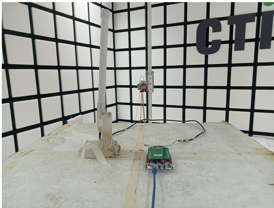
Radiated spurious emission Test Setup-2(Above 1GHz)-2
