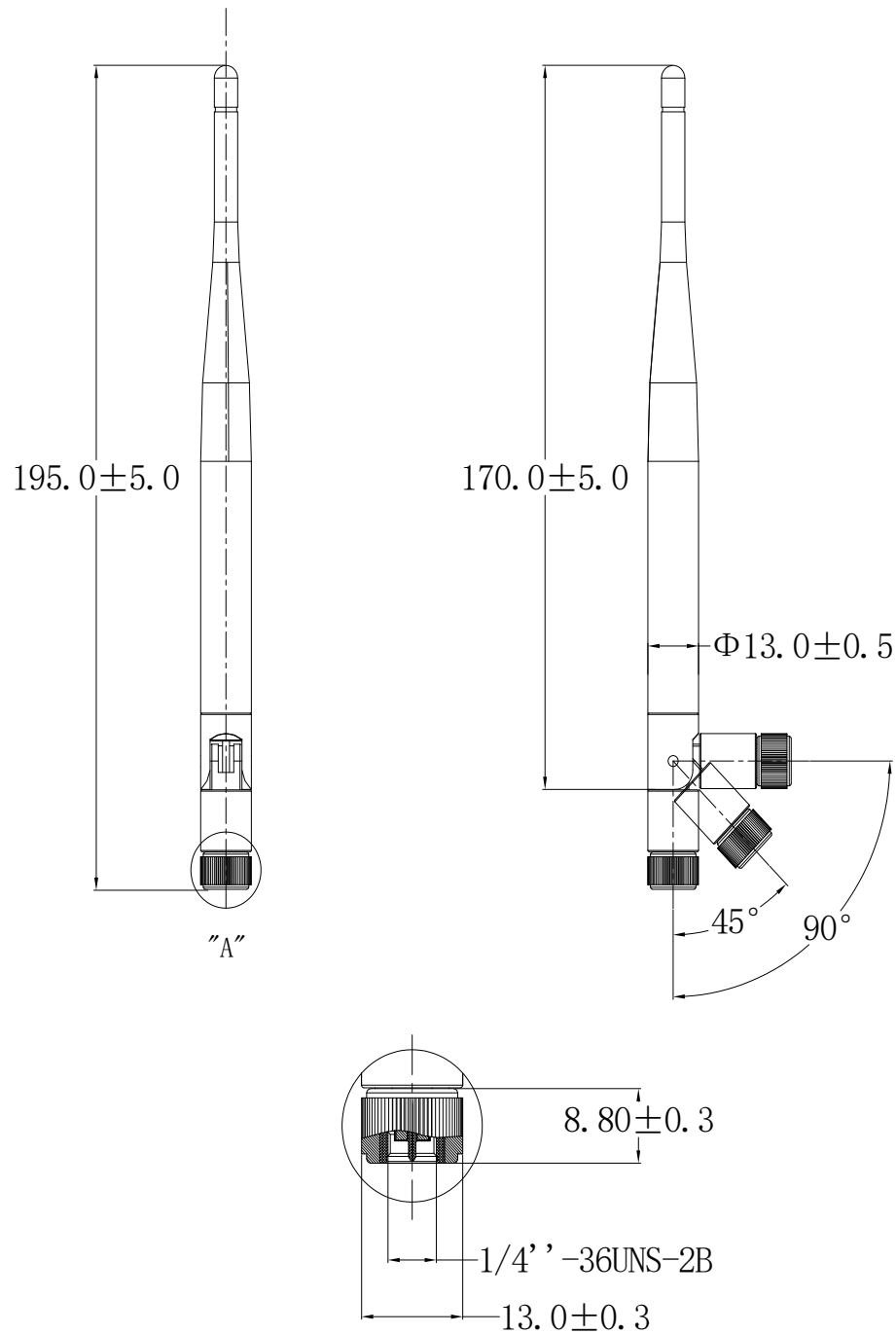
SMA-Male DETAIL A
