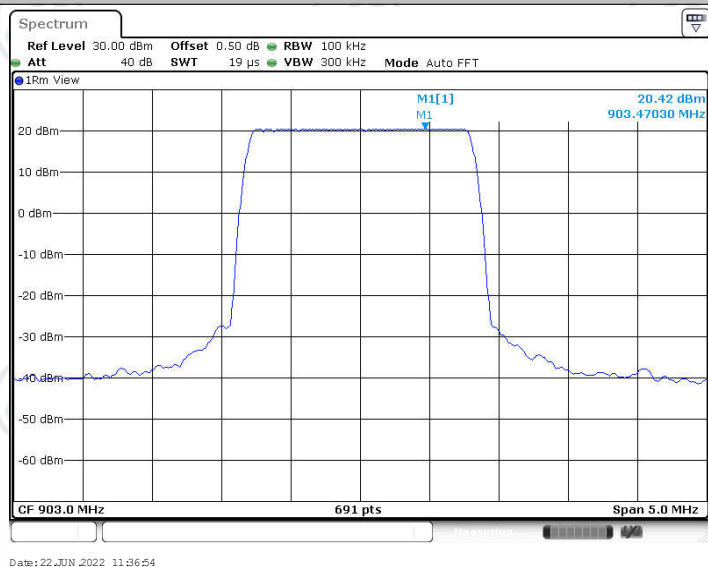
BW1523.4K_Ant1_903_0-Reference
