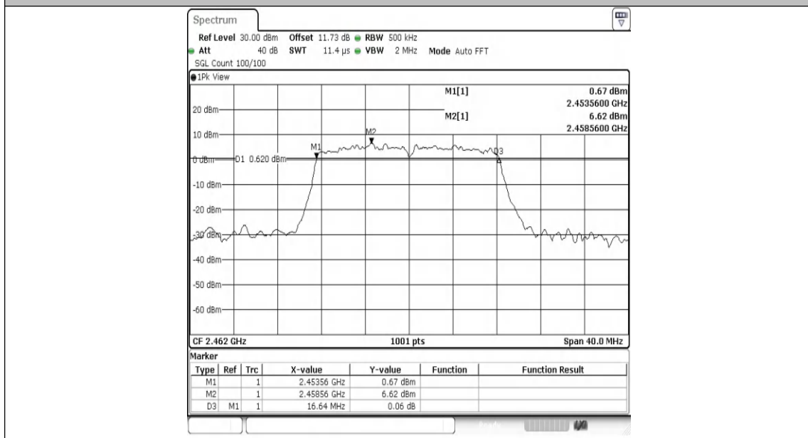
11G-Ant1-2462-PASS
