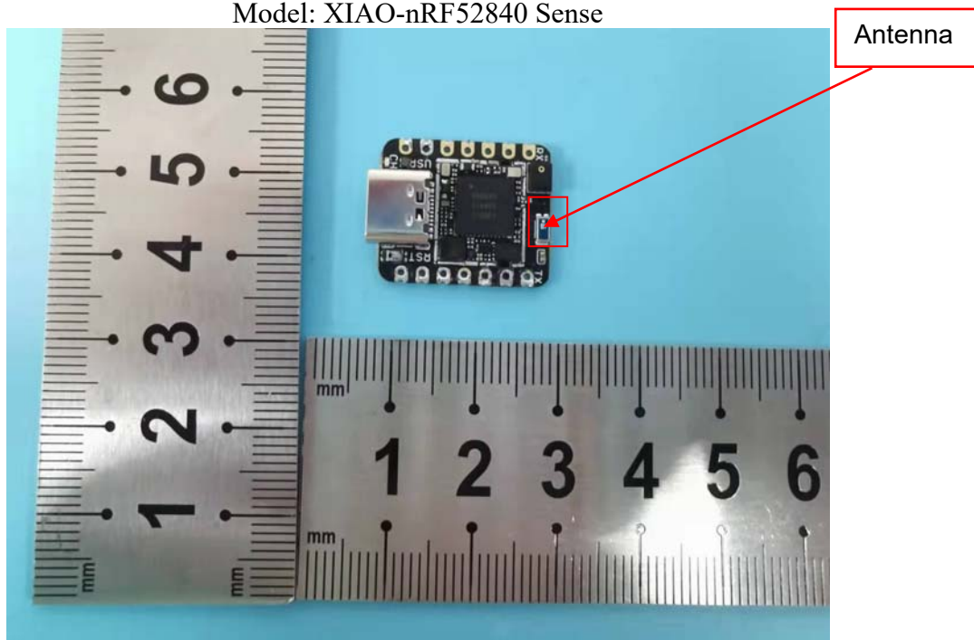
Internal photos Model: XIAO-nRF52840 Sense
