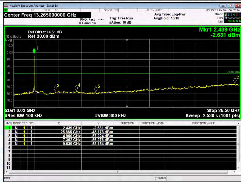
Tx. Spurious NVNT n(HT40) 2442MHz Ant1 Emission
