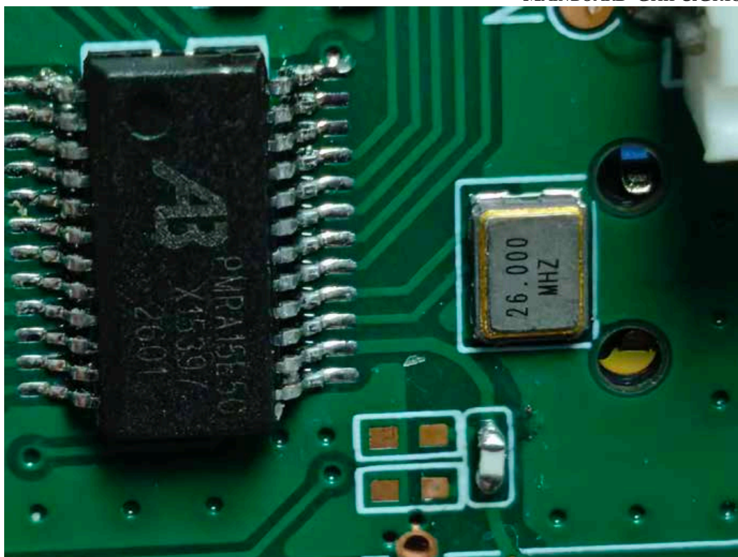
FIGURE 24 BAUHN KMA-1 KARAOKE MICROPHONE ASSORTMENT (BKM-20) (M/N: BKM-20 SILVER) MAINBOARD-CHIP&CRYSTAL
