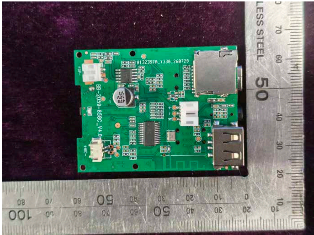
FIGURE 22 BAUHN KMA-1 KARAOKE MICROPHONE ASSORTMENT (BKM-20) (M/N: BKM-20 SILVER) MAINBOARD FRONT
