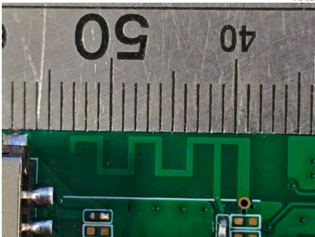
FIGURE 25 BAUHN KMA-1 KARAOKE MICROPHONE ASSORTMENT (BKM-20) (M/N: BKM-20 SILVER) ANTENNA
