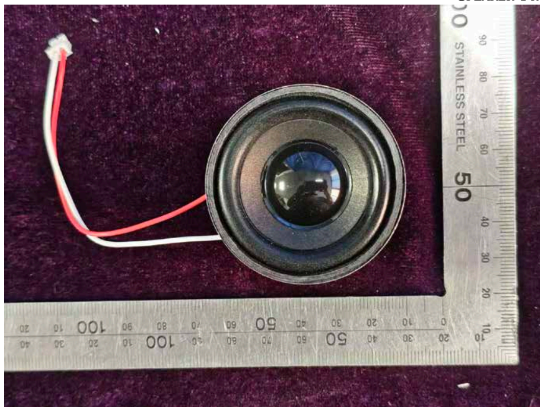
FIGURE 26 BAUHN KMA-1 KARAOKE MICROPHONE ASSORTMENT (BKM-20) (M/N: BKM-20 SILVER) SPEAKER FRONT
