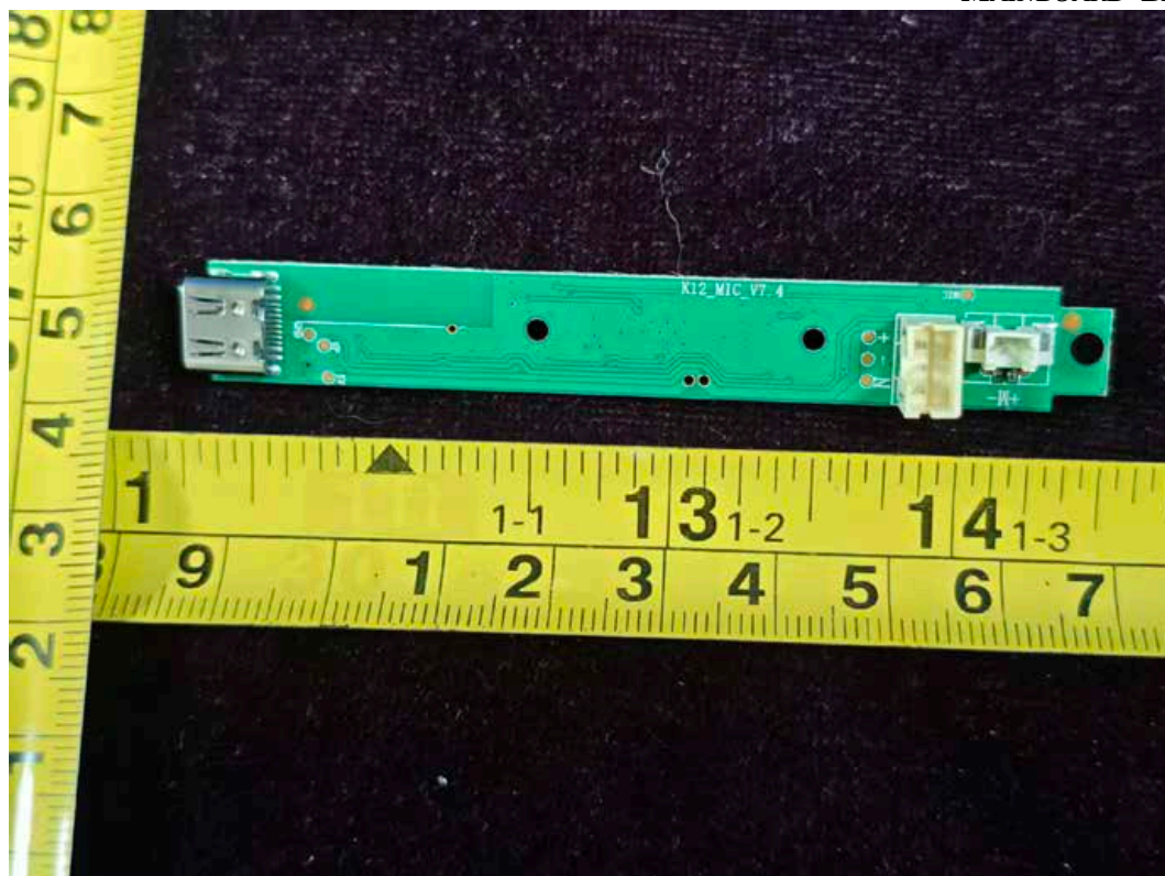
FIGURE 16 BAUHN KMA-1 KARAOKE MICROPHONE ASSORTMENT (BKS-30) (M/N: BKS-30 BLACK) MAINBOARD BACK
