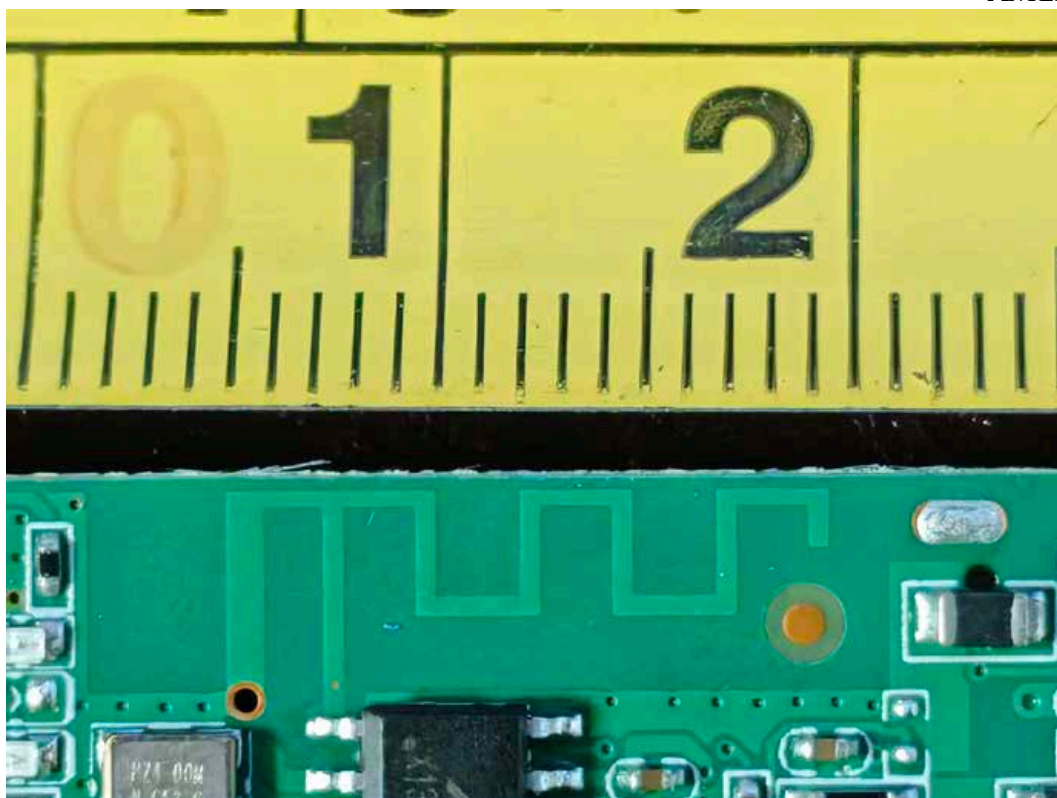
FIGURE 18 BAUHN KMA-1 KARAOKE MICROPHONE ASSORTMENT (BKS-30) (M/N: BKS-30 BLACK) ANTENNA
