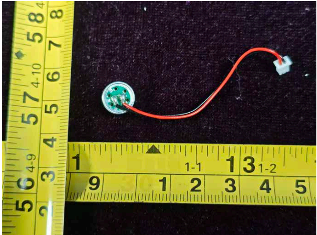
FIGURE 20 BAUHN KMA-1 KARAOKE MICROPHONE ASSORTMENT (BKS-30) (M/N: BKS-30 BLACK) MIC BACK
