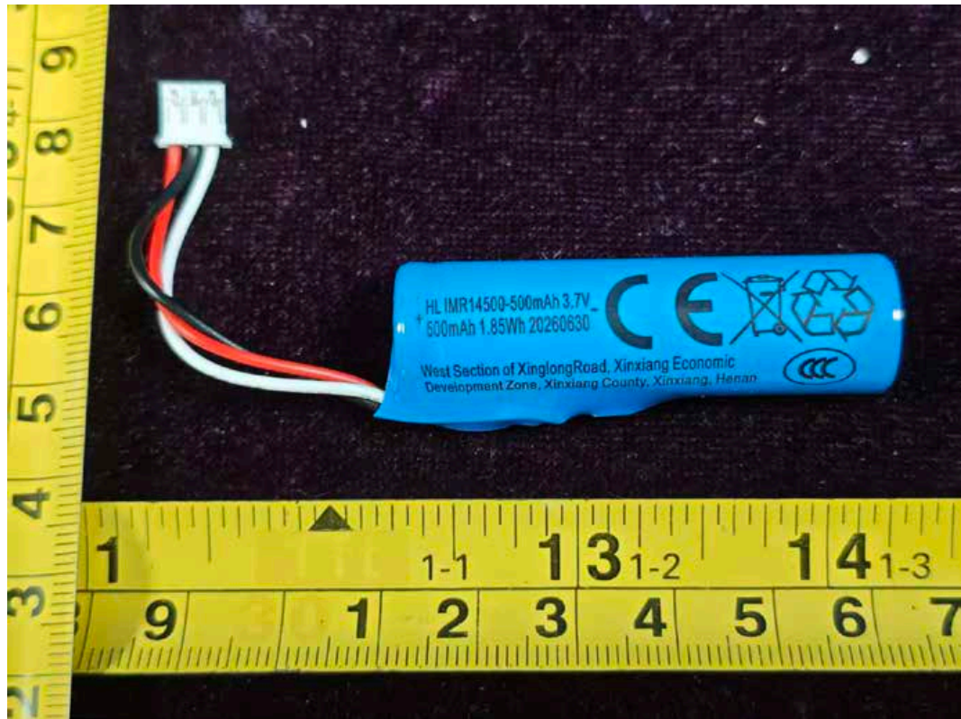
FIGURE 21 BAUHN KMA-1 KARAOKE MICROPHONE ASSORTMENT (BKS-30) (M/N: BKS-30 BLACK) BATTERY
