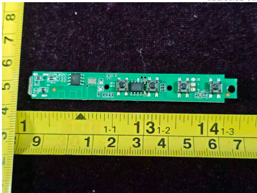
FIGURE 15 BAUHN KMA-1 KARAOKE MICROPHONE ASSORTMENT (BKS-30) (M/N: BKS-30 BLACK) MAINBOARD FRONT
