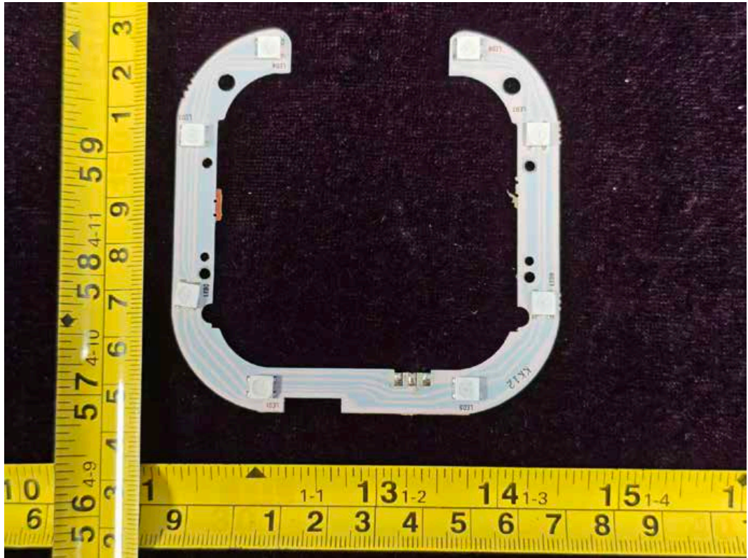
FIGURE 21 BAUHN KMA-1 KARAOKE MICROPHONE ASSORTMENT (BKS-30) (M/N: BKS-30 BLACK) LEDBOARD FRONT
