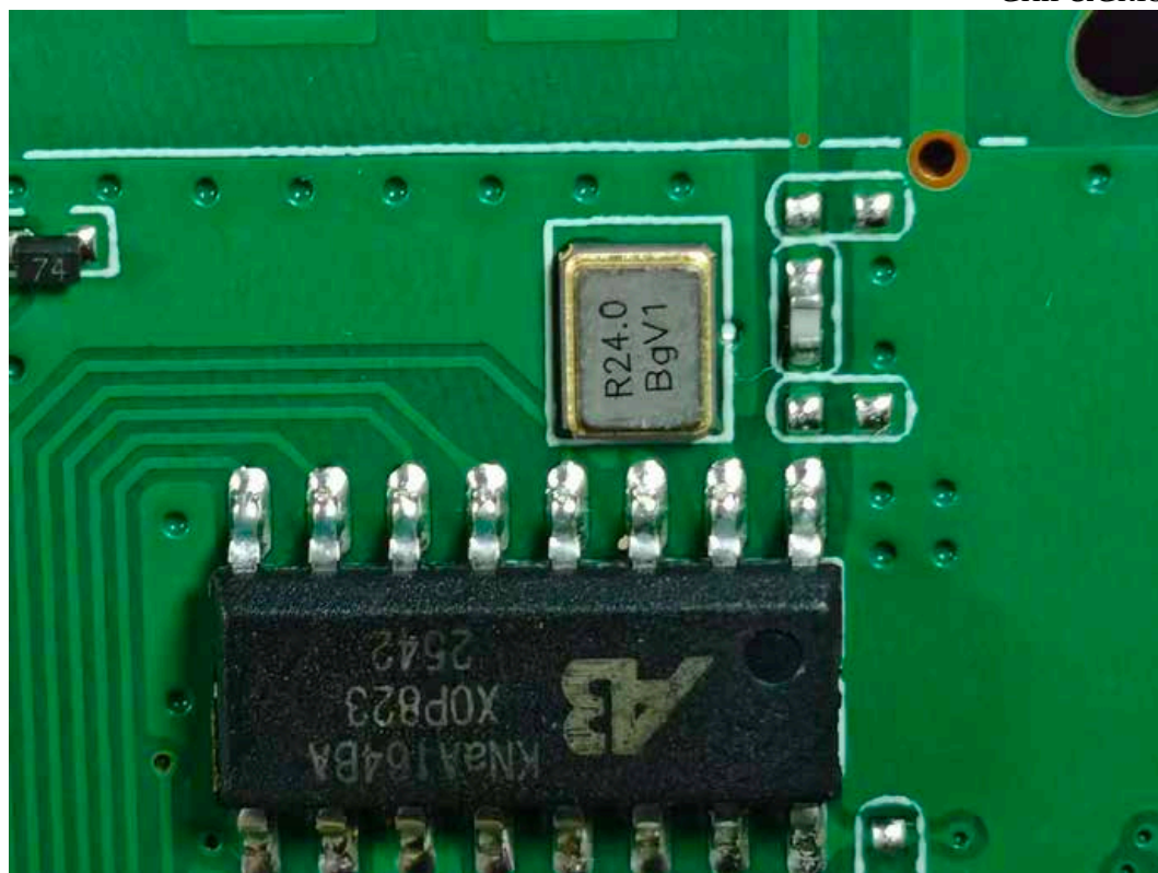
FIGURE 19 BAUHN KMA-1 KARAOKE MICROPHONE ASSORTMENT (BKS-30) (M/N: BKS-30 BLACK) CHIP&CRYSTAL
