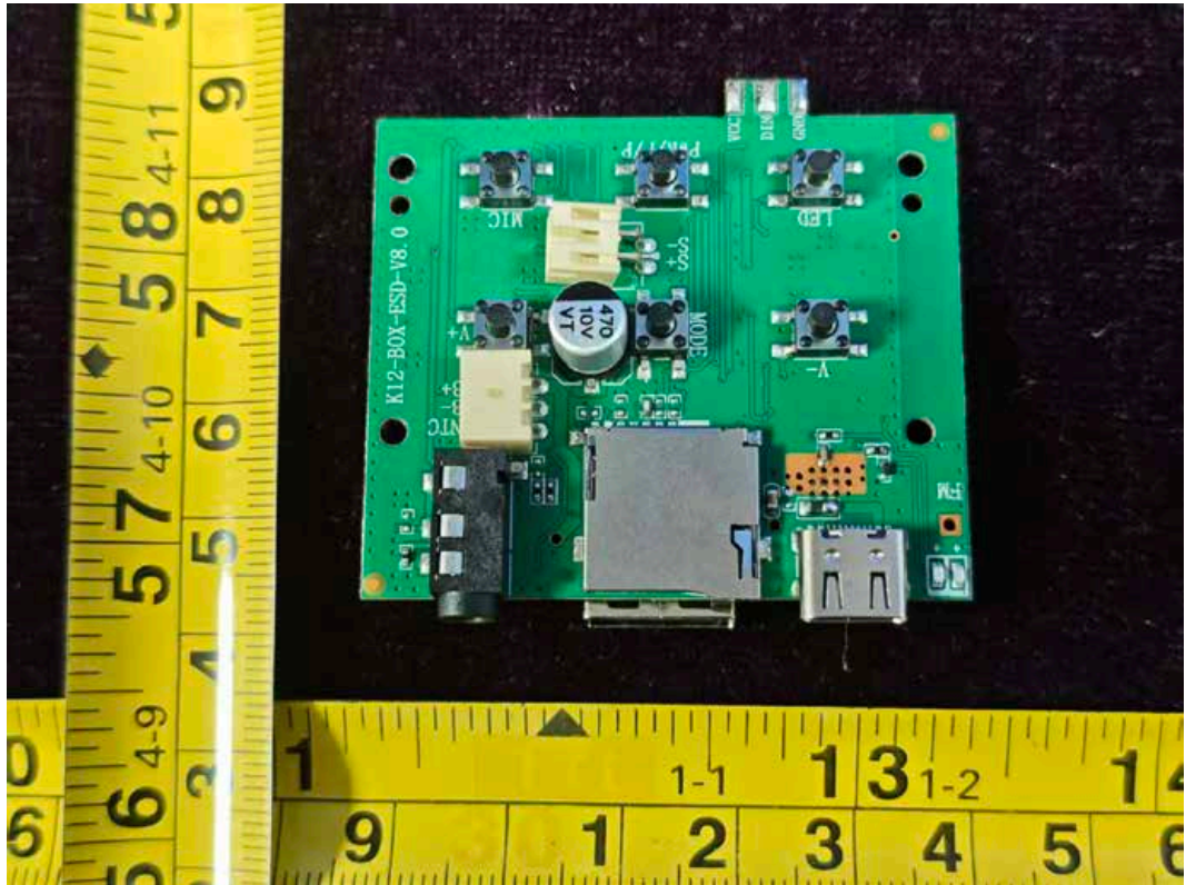
FIGURE 17 BAUHN KMA-1 KARAOKE MICROPHONE ASSORTMENT (BKS-30) (M/N: BKS-30 BLACK) MAINBOARD FRONT
