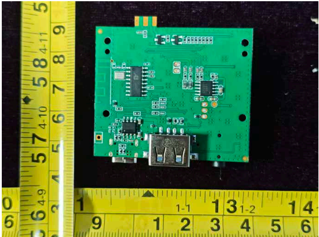
FIGURE 18 BAUHN KMA-1 KARAOKE MICROPHONE ASSORTMENT (BKS-30) (M/N: BKS-30 BLACK) MAINBOARD BACK
