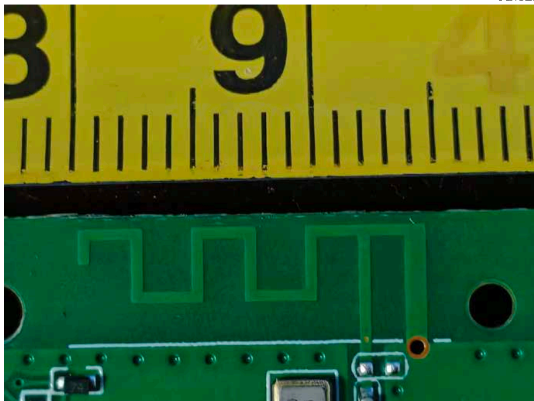
FIGURE 20 BAUHN KMA-1 KARAOKE MICROPHONE ASSORTMENT (BKS-30) (M/N: BKS-30 BLACK) ANTENNA
