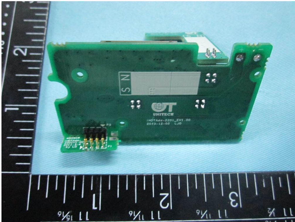
Connect board 6 - Rear View
