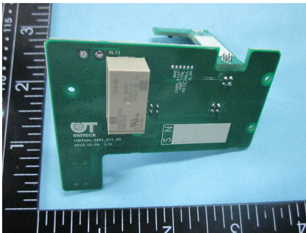
Connect board 5 - Rear View
