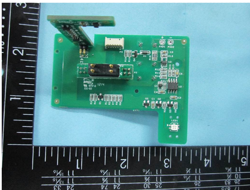
Connect board 5 - Front View
