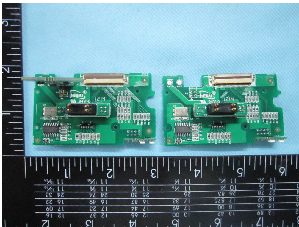
Two Same Connect board 6 - Front View
