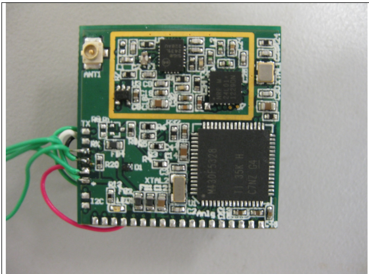
Model SD2, Top View with Shield Removed
