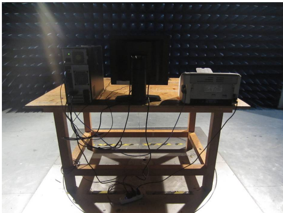
RE TEST SETUP OF C16S-4
