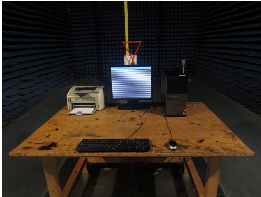
RE TEST SETUP OF C16S-3
