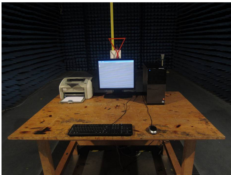
RE TEST SETUP SAMPLE-C16S-3
