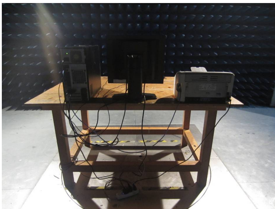
RE TEST SETUP SAMPLE-C16S-4
