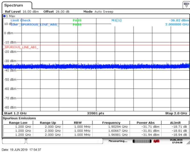
Figure 6.5-20: Conducted Spurious Emissions above 1.2 GHz, Tx @mid channel 50W 7k60FXW modulation
