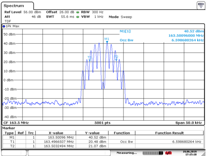
Figure 6.3-1: Occupied Bandwidth, Tx @mid channel 50 W 7k60FXW modulation
