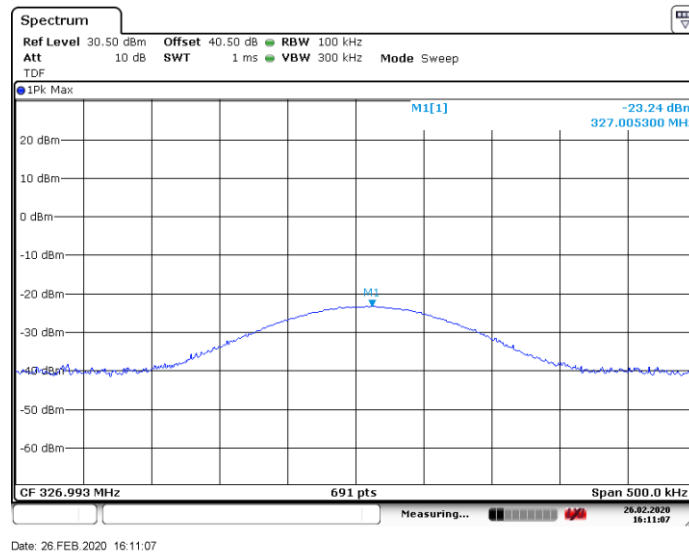
Figure 6.5-27: Conducted Spurious Emissions @326.993 MHz, Tx @mid channel 50W 6k00F3E modulation
