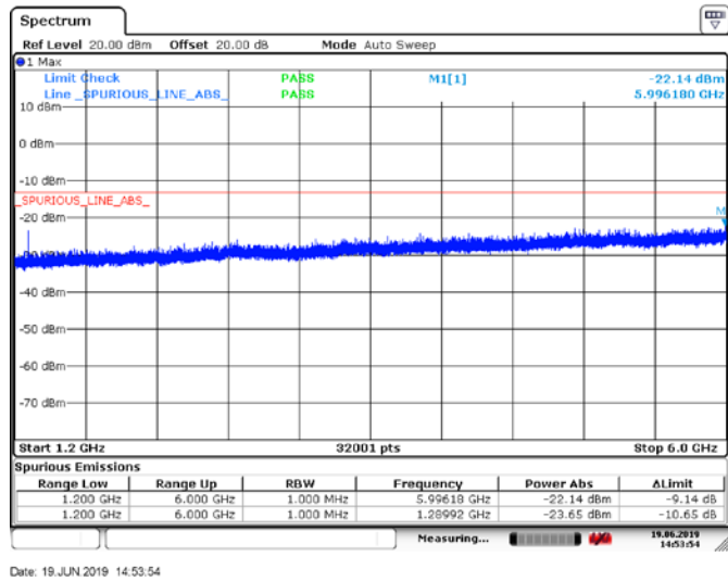
Figure 6.5-9: Conducted Spurious Emissions above 1.2 GHz, Tx @Low channel of 420 MHz band, 10W 25kHzTEDS modulation
