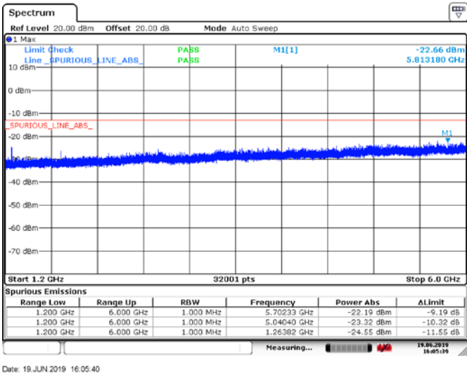
Figure 6.5-2: Conducted Spurious Emissions above 1.2 GHz, Tx @Low channel of 420 MHz band, 50W 7k60FXW modulation
