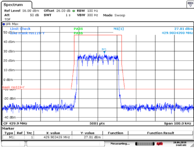
Figure 6.4-26: Mask y, Tx @high channel of 420 MHz band, 10 W 25kHzTEDS modulation
