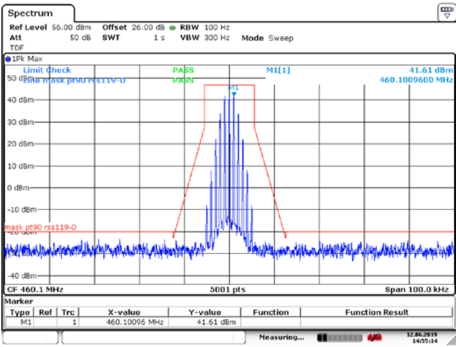
Figure 6.4-11: Mask d, Tx @low channel of 460 MHz band, 50W 11kF3E modulation
