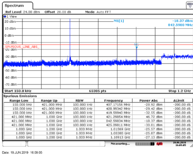
Figure 6.5-6: Conducted Spurious Emissions below 1.2 GHz, Tx @Low channel of 420 MHz band, 25W 0.35TETRA modulation
