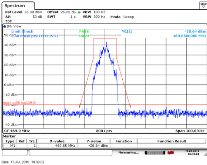
Figure 6.4-4: Mask d, Tx @low channel of 460 MHz band, 50W 7k60FXW modulation
