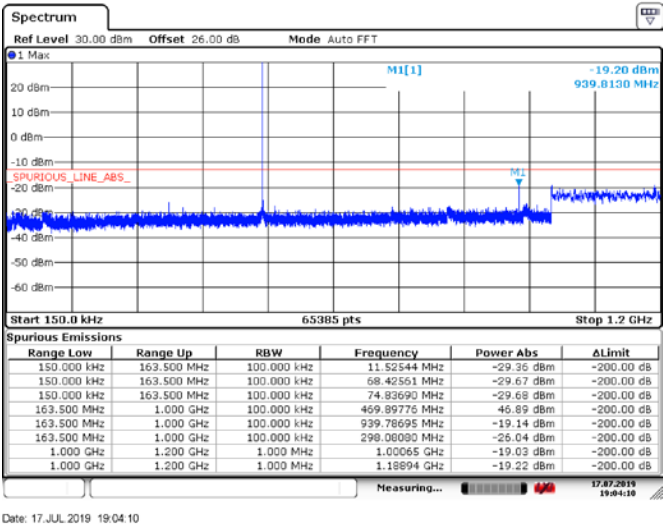
Figure 6.5-31: Conducted Spurious Emissions below 1.2 GHz, Tx @high channel of 460 MHz band, 50W 16kF3E modulation
