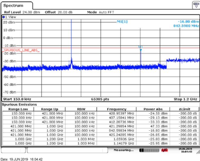
Figure 6.5-1: Conducted Spurious Emissions below 1.2 GHz, Tx @Low channel of 420 MHz band, 50W 7k60FXW modulation
