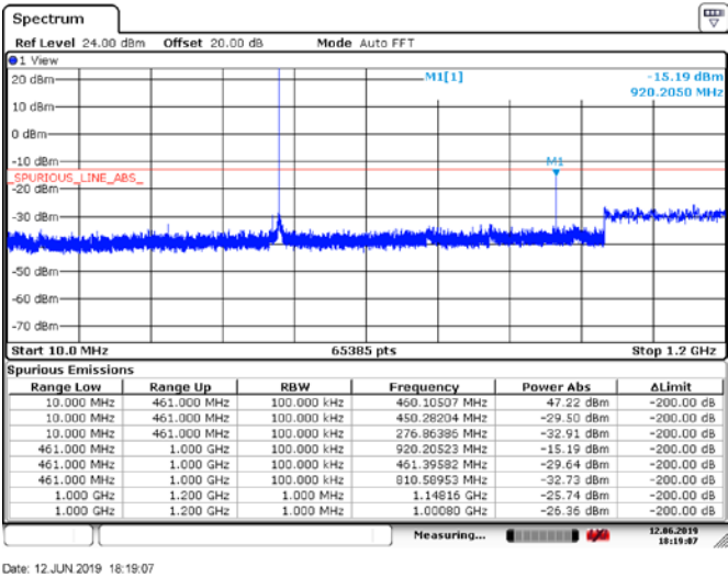
Figure 6.5-22: Conducted Spurious Emissions below 1.2 GHz, Tx @ low channel of 460 MHz band, 50W 16k0F3E modulation
