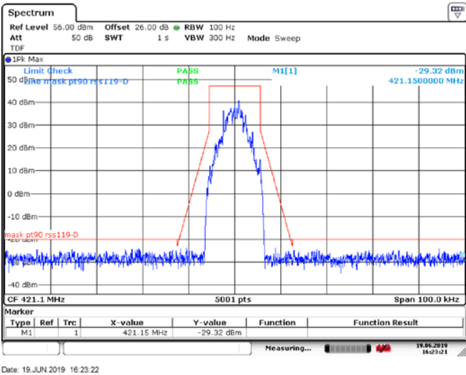
Figure 6.4-1: Mask d, Tx @low channel of 420 MHz band, 50W 7k60FXW modulation
