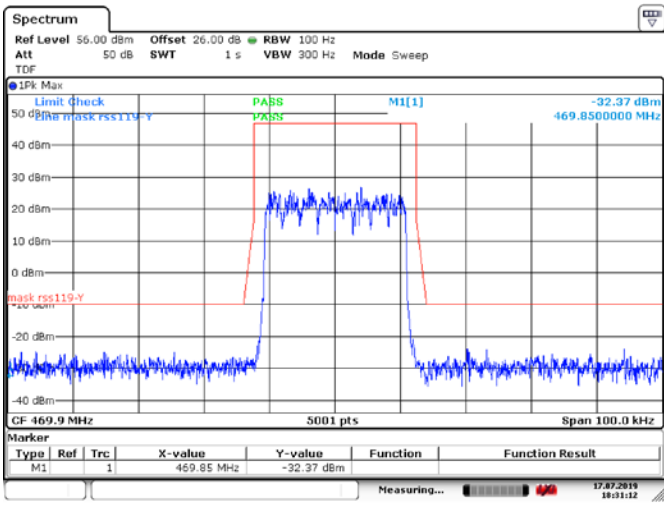
Figure 6.4-28: Mask y, Tx @low channel of 460 MHz band, 10 W 25kHzTEDS modulation
