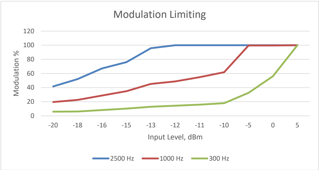
Figure 6.2-2: Modulation Limiting, modulation 16kF3E
