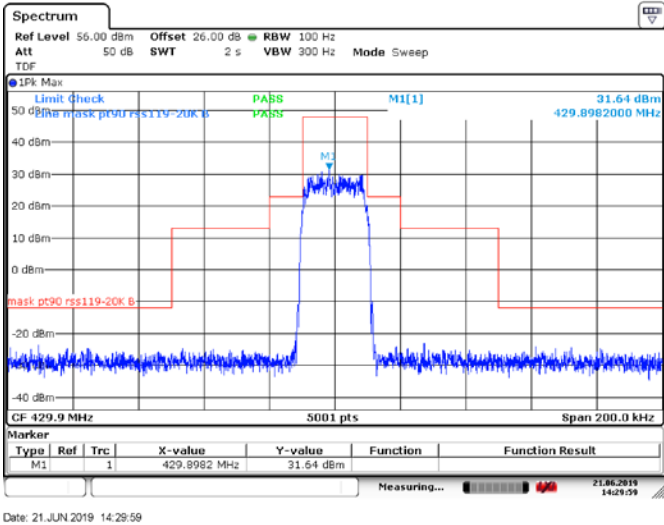
Figure 6.4-18: Mask b, Tx @high channel of 420 MHz band, 25 W 0.20TETRA modulation
