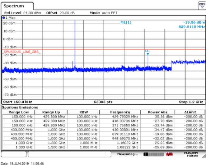
Figure 6.5-17: Conducted Spurious Emissions below 1.2 GHz, Tx @high channel of 420 MHz band, 10W 25kHzTEDS modulation
