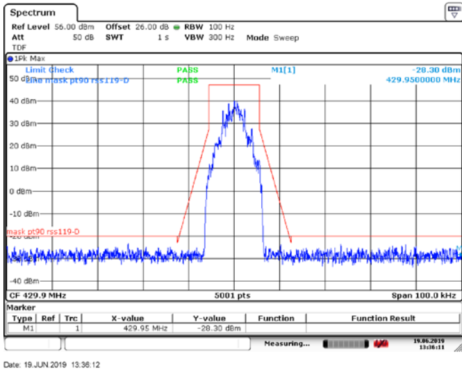
Figure 6.4-2: Mask d, Tx @high channel of 420 MHz band, 50W 7k60FXW modulation
