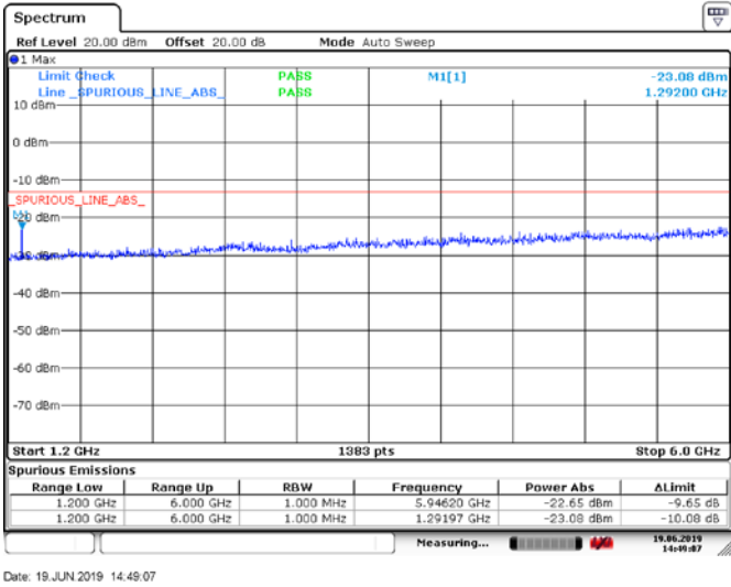
Figure 6.5-14: Conducted Spurious Emissions above 1.2 GHz, Tx @high channel of 420 MHz band, 50W 16kOF3E modulation
