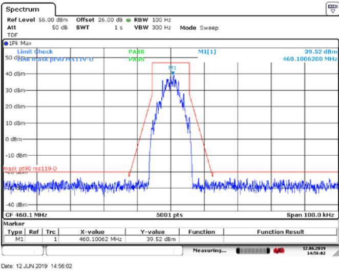
Figure 6.4-3: Mask d, Tx @low channel of 460 MHz band, 50W 7k60FXW modulation
