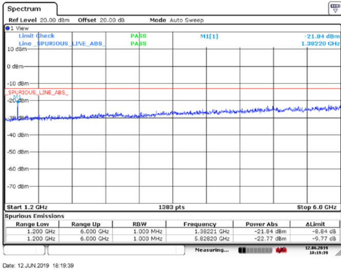
Figure 6.5-23: Conducted Spurious Emissions above 1.2 GHz, Tx @ low channel of 460 MHz band, 50W 16k0F3E modulation
