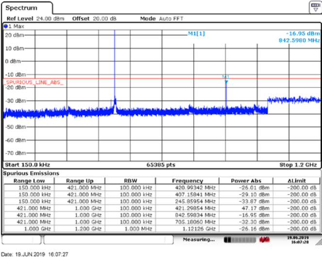
Figure 6.5-4: Conducted Spurious Emissions below 1.2 GHz, Tx @Low channel of 420 MHz band, 50W 16Kof3E modulation
