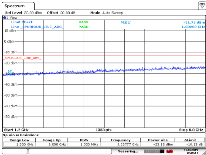
Figure 6.5-20: Conducted Spurious Emissions above 1.2 GHz, Tx @ low channel of 460 MHz band, 50W o. 7k60FXW modulation
