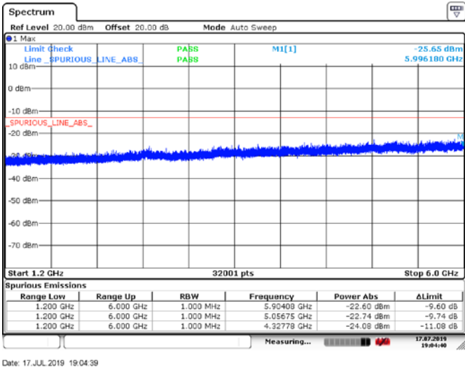
Figure 6.5-32: Conducted Spurious Emissions above 1.2 GHz, Tx @high channel of 460 MHz band, 50W 16kF3E modulation
