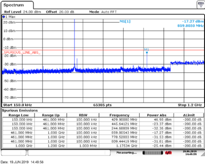
Figure 6.5-13: Conducted Spurious Emissions below 1.2 GHz, Tx @high channel of 420 MHz band, 50W 16kOF3E modulation
