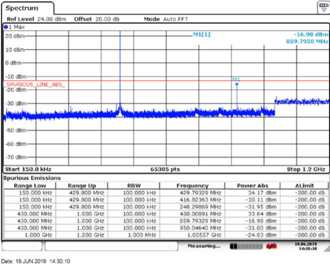
Figure 6.5-10: Conducted Spurious Emissions below 1.2 GHz, Tx @high channel of 420 MHz band, 50W 7k60FXW modulation
