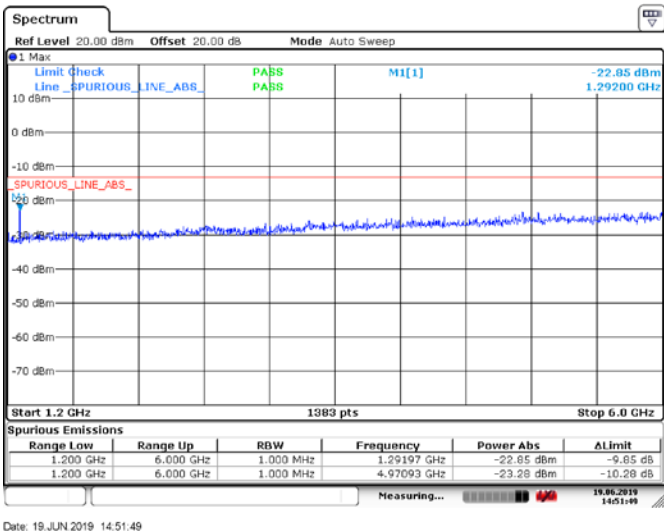
Figure 6.5-16: Conducted Spurious Emissions above 1.2 GHz, Tx @high channel of 420 MHz band, 25W 0.35TETRA modulation
