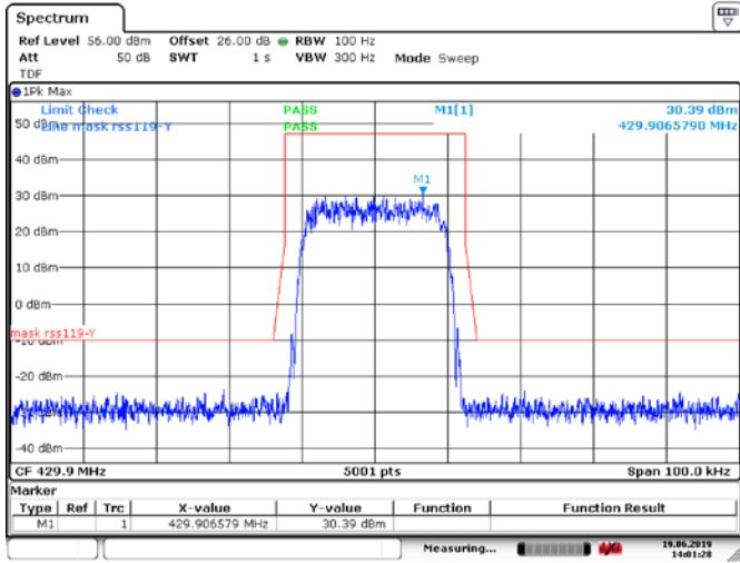
Figure 6.4-22: Mask y, Tx @high channel of 420 MHz band, 25 W o. 35TETRA modulation
