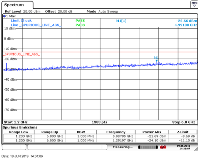
Figure 6.5-11: Conducted Spurious Emissions above 1.2 GHz, Tx @high channel of 420 MHz band, 50W o. 7k60FXW modulation
