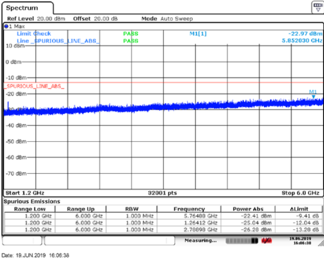
Figure 6.5-5: Conducted Spurious Emissions above 1.2 GHz, Tx @Low channel of 420 MHz band, 50W 16Kof3E modulation
