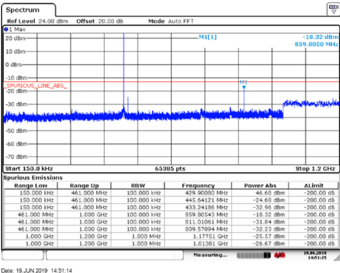
Figure 6.5-15: Conducted Spurious Emissions below 1.2 GHz, Tx @high channel of 420 MHz band, 25W 0.35TETRA modulation
