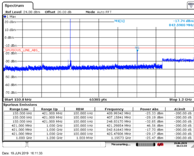
Figure 6.5-8: Conducted Spurious Emissions below 1.2 GHz, Tx @Low channel of 420 MHz band, 10W 25kHzTEDS modulation
