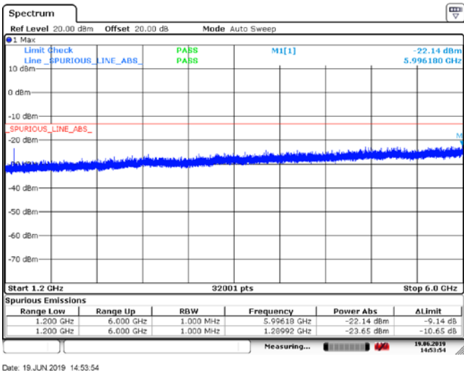
Figure 6.5-18: Conducted Spurious Emissions above 1.2 GHz, Tx @high channel of 420 MHz band, 10W 25kHzTEDS modulation
