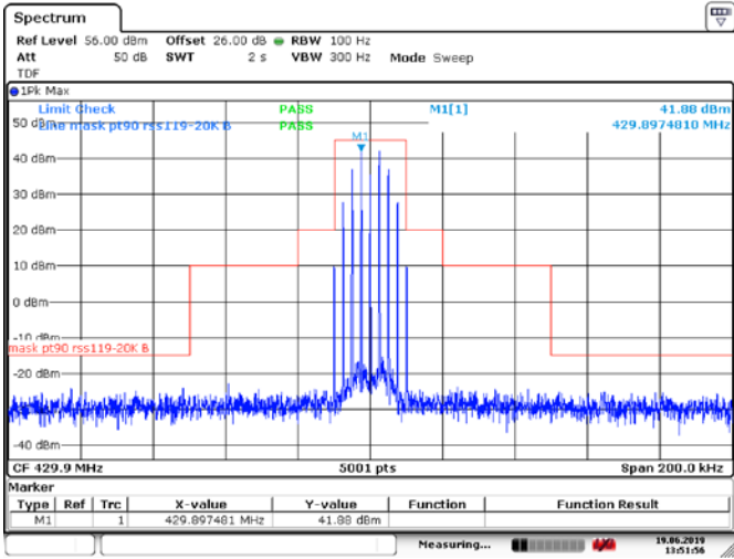
Figure 6.4-6: Mask b, Tx @high channel of 420 MHz band, 50W 16kF3E modulation
