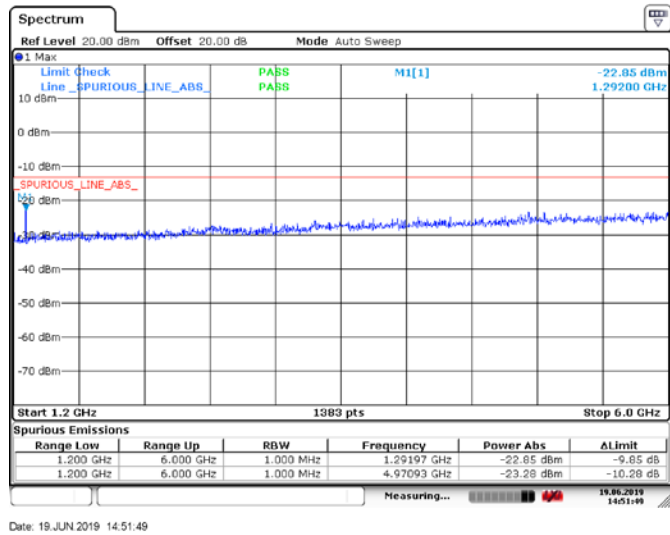
Figure 6.5-7: Conducted Spurious Emissions above 1.2 GHz, Tx @Low channel of 420 MHz band, 25W 0.35TETRA modulation
