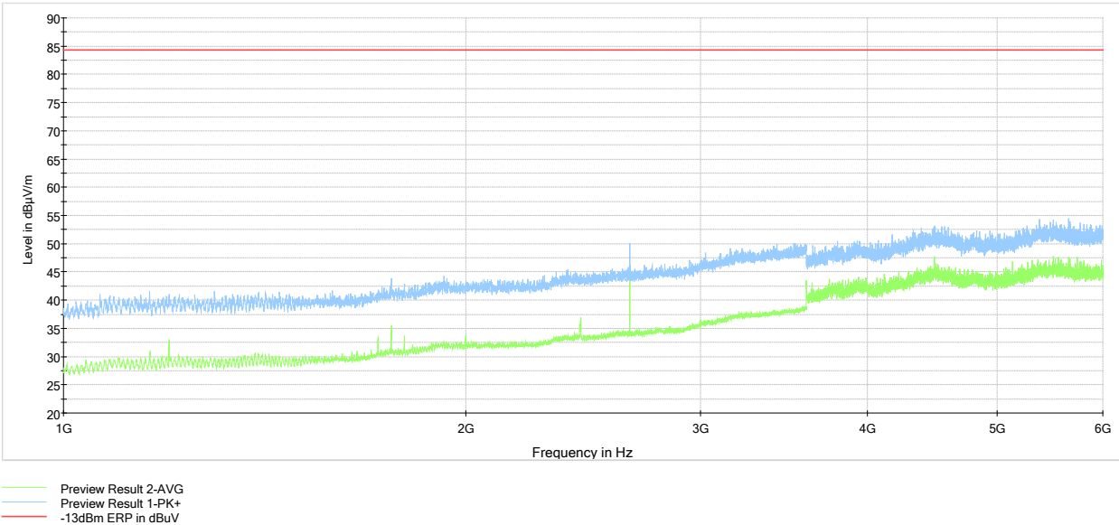
Figure 6.6-22: Cabinet Radiated Spurious Emissions above 1 GHz, Tx @low channel of 460 MHz band, 25W 0.35TETRA modulation
