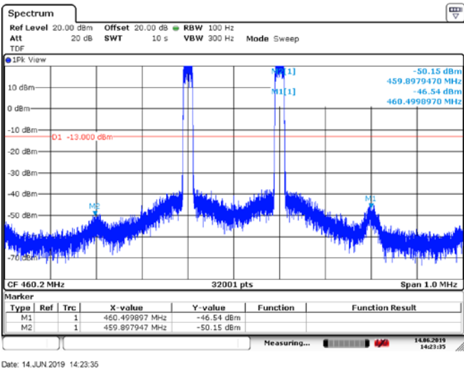
Figure 6.5-47: Conducted Spurious Emissions from inter-modulation products, Tx @low channel of 460 MHz band, 2X10W 0.35TETRA modulation
