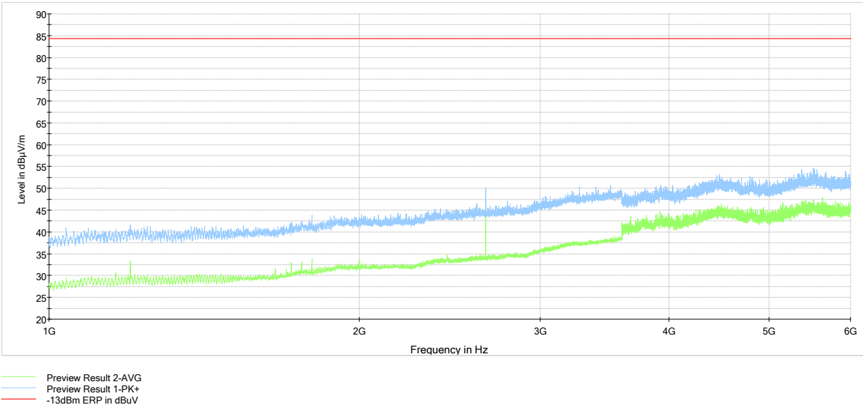
Figure 6.6-20: Cabinet Radiated Spurious Emissions above 1 GHz, Tx @low channel of 460 MHz band, 50W 16Kof3E modulation
