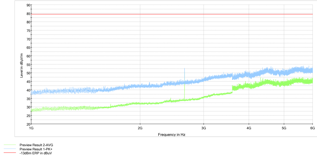
Figure 6.6-14: Cabinet Radiated Spurious Emissions above 1 GHz, Tx @ high channel of 420 MHz band, 25W 0.35TETRA modulation
