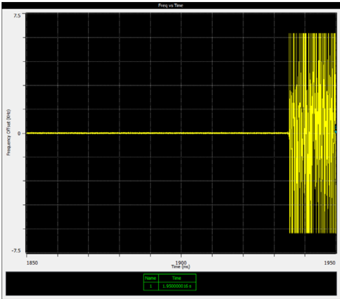
Figure 6.7-5: Transient Frequency behavior, Tx @ mid channel 6.25 k channel, switch ON
