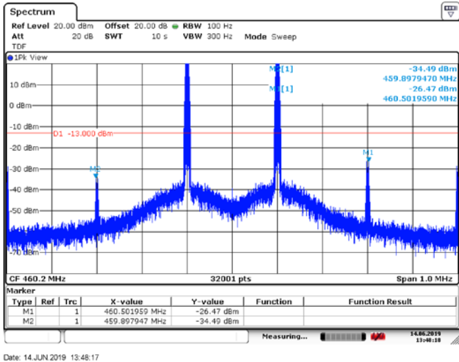
Figure 6.5-46: Conducted Spurious Emissions from inter-modulation products, Tx @low channel of 460 MHz band, 2X15W 16K0F3E modulation
