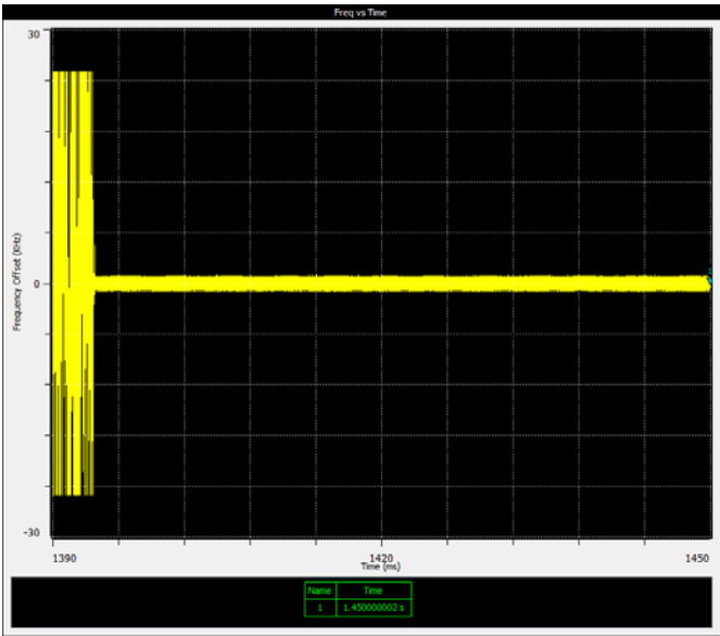
Figure 6.7-1: Transient Frequency behavior, Tx @ mid channel 25 k channel, switch ON
