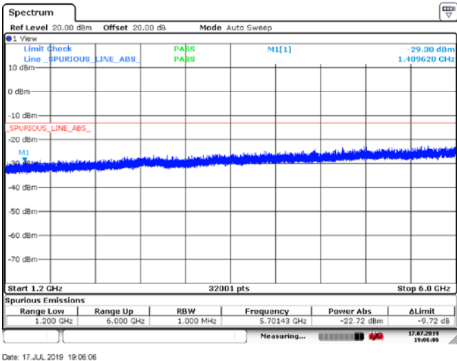
Figure 6.5-36: Conducted Spurious Emissions above 1.2 GHz, Tx @high channel of 460 MHz band, 10W 25kHzTEDS modulation
