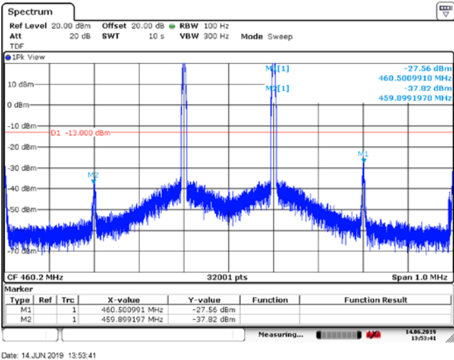
Figure 6.5-45: Conducted Spurious Emissions from inter-modulation products, Tx @low channel of 460 MHz band, 2X15W 7k60FXW modulation
