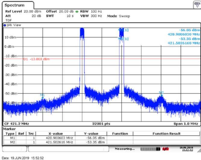
Figure 6.5-40: Conducted Spurious Emissions from inter-modulation products, Tx @low channel of 420 MHz band, 2X7W 25kHzTEDS modulation
