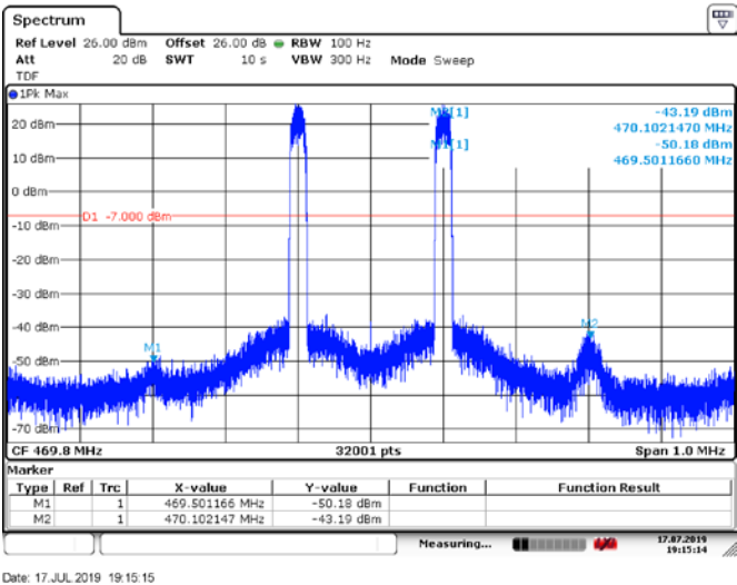
Figure 6.5-51: Conducted Spurious Emissions from inter-modulation products, Tx @ high channel of 460 MHz band, 2X10W 0.35TETRA modulation
