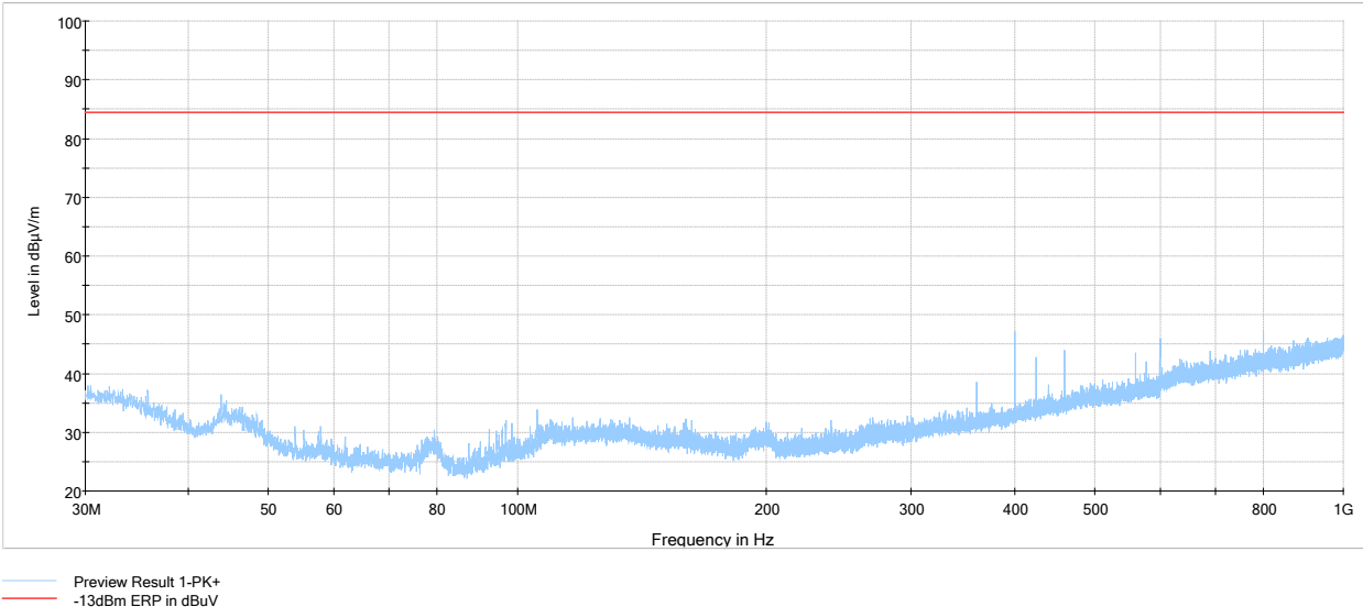
Figure 6.6-21: Cabinet Radiated Spurious Emissions below 1 GHz, Tx @low channel of 460 MHz band, 25W 0.35TETRA modulation
