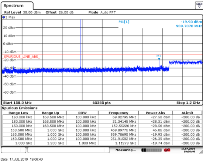
Figure 6.5-35: Conducted Spurious Emissions below 1.2 GHz, Tx @high channel of 460 MHz band, 10W 25kHzTEDS modulation
