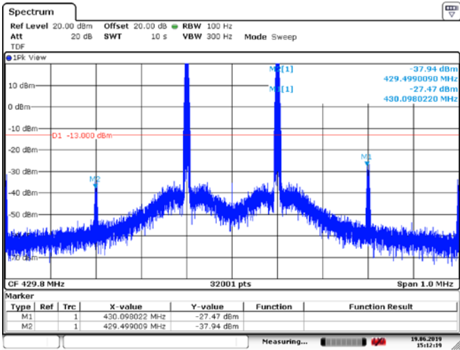
Figure 6.5-42: Conducted Spurious Emissions from inter-modulation products, Tx @ high channel of 420 MHz band, 2X15W 16K0F3E modulation
