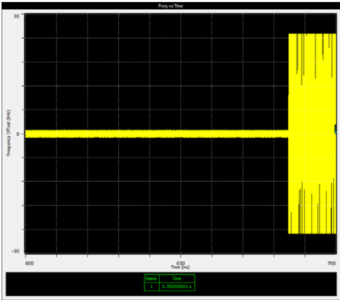
Figure 6.7-2: Transient Frequency behavior, Tx @ mid channel 25 k channel, switch OFF
