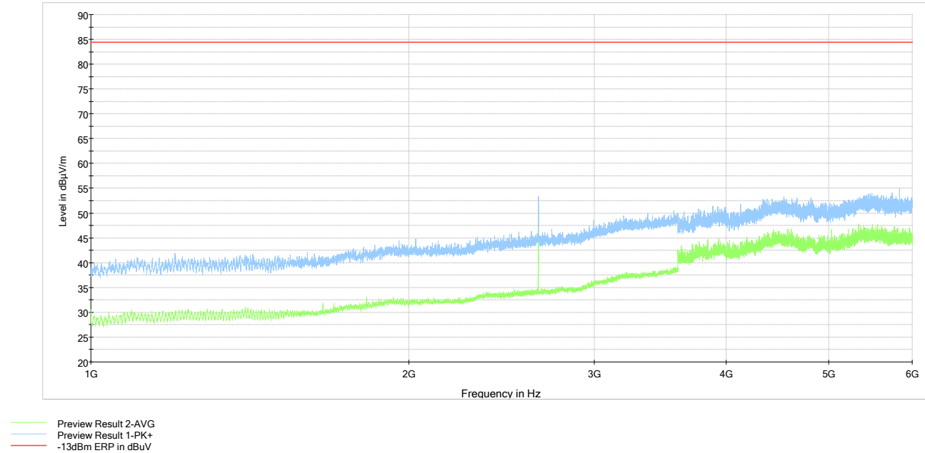
Figure 6.6-10: Cabinet Radiated Spurious Emissions above 1 GHz, Tx @ high channel of 420 MHz band, 50W 7k60FXW modulation
