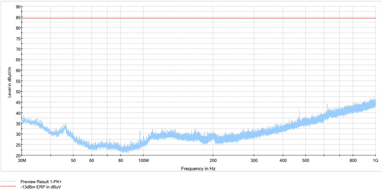
Figure 6.6-29: Cabinet Radiated Spurious Emissions below 1 GHz, Tx @ high channel of 460 MHz band, 25W 0.35TETRA modulation
