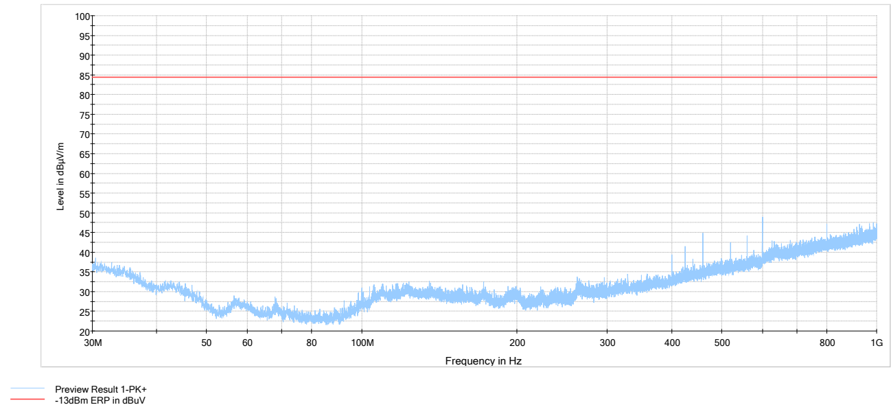
Figure 6.6-17: Cabinet Radiated Spurious Emissions below 1 GHz, Tx @low channel of 460 MHz band, 50W 7k60FXW modulation
