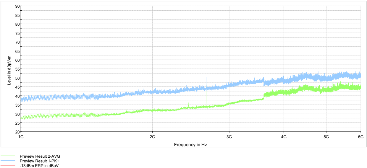
Figure 6.6-26: Cabinet Radiated Spurious Emissions above 1 GHz, Tx @ high channel of 460 MHz band, 50W 7k60FXW modulation
