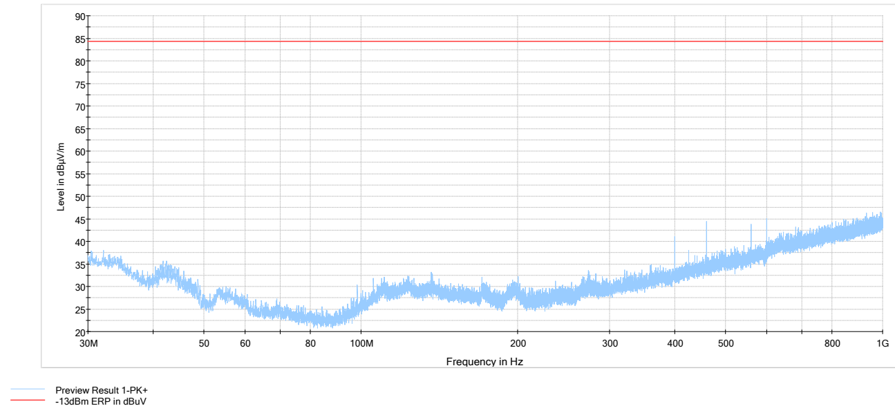
Figure 6.6-19: Cabinet Radiated Spurious Emissions below 1 GHz, Tx @low channel of 460 MHz band, 50W 16Kof3E modulation
