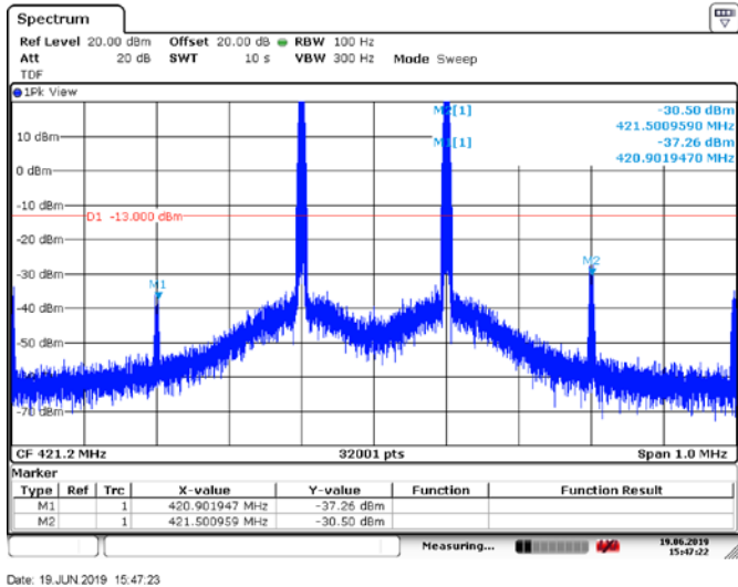
Figure 6.5-38: Conducted Spurious Emissions from inter-modulation products, Tx @low channel of 420 MHz band, 2X15W 16Kof3E modulation
