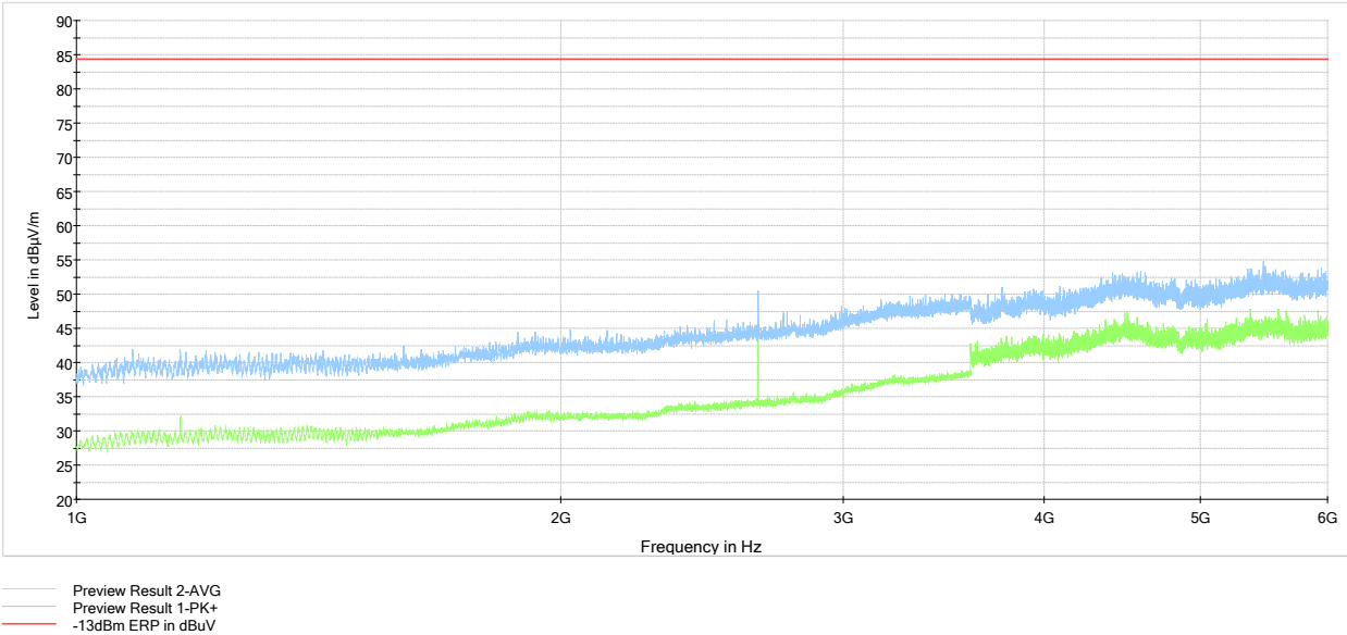
Figure 6.6-30: Cabinet Radiated Spurious Emissions above 1 GHz, Tx @ high channel of 460 MHz band, 25W 0.35TETRA modulation
