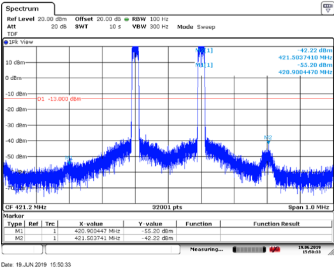
Figure 6.5-39: Conducted Spurious Emissions from inter-modulation products, Tx @low channel of 420 MHz band, 2X10W 0.35TETRA modulation
