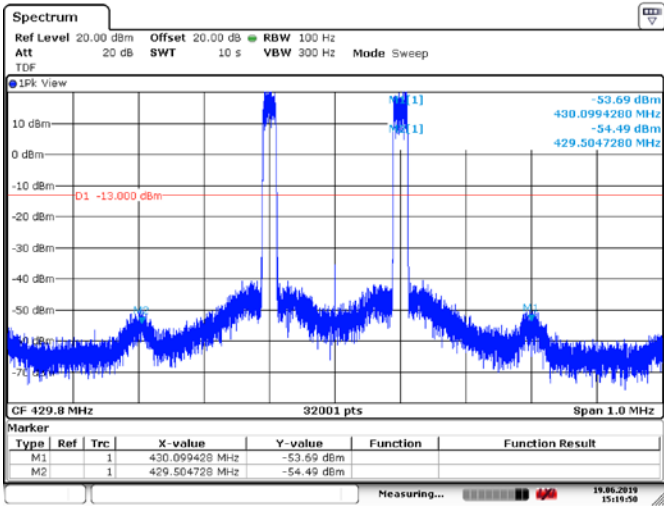
Figure 6.5-44: Conducted Spurious Emissions from inter-modulation products, Tx @ high channel of 420 MHz band, 2X7W 25kHzTEDS modulation
