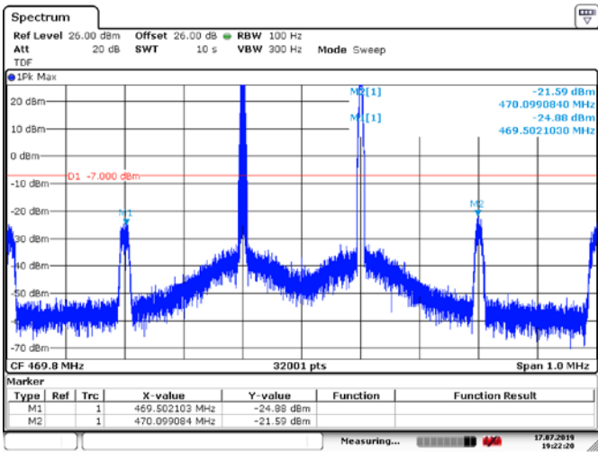
Figure 6.5-50: Conducted Spurious Emissions from inter-modulation products, Tx @ high channel of 460 MHz band, 2X15W 16K0F3E modulation
