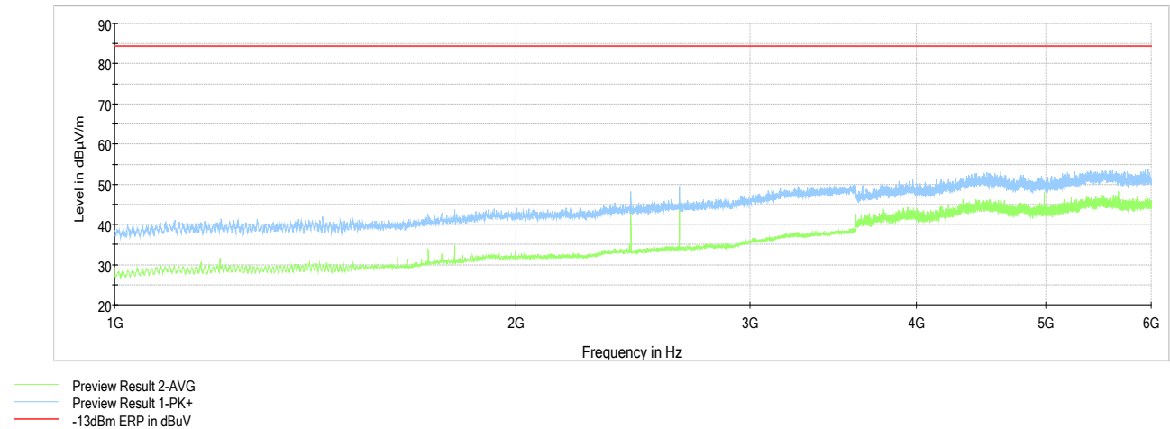
Figure 6.6-18: Cabinet Radiated Spurious Emissions above 1 GHz, Tx @low channel of 460 MHz band, 50W 7k60FXW modulation
