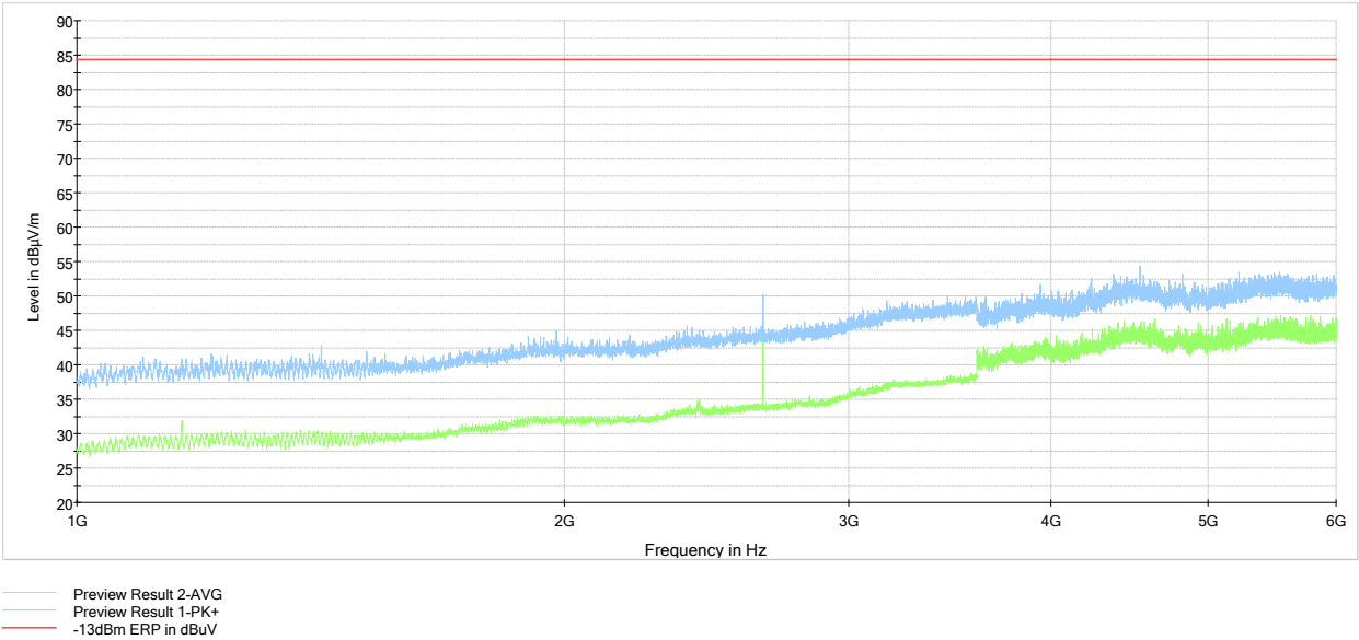
Figure 6.6-28: Cabinet Radiated Spurious Emissions above 1 GHz, Tx @ high channel of 460 MHz band, 50W 16KoF3E modulation
