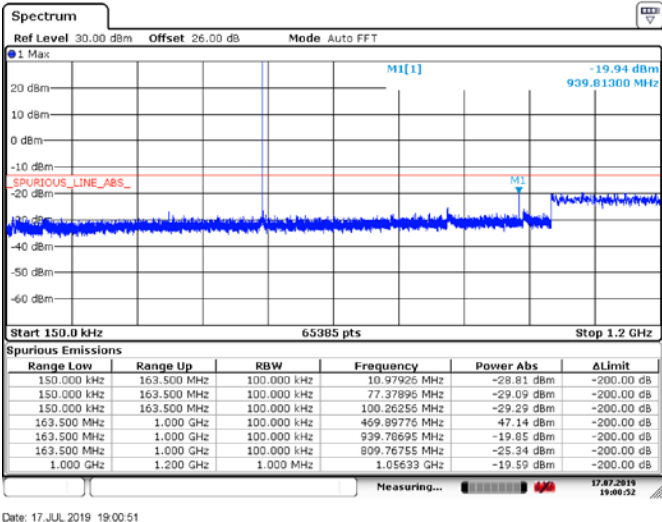
Figure 6.5-33: Conducted Spurious Emissions below 1.2 GHz, Tx @high channel of 460 MHz band, 25W 0.35TETRA modulation
