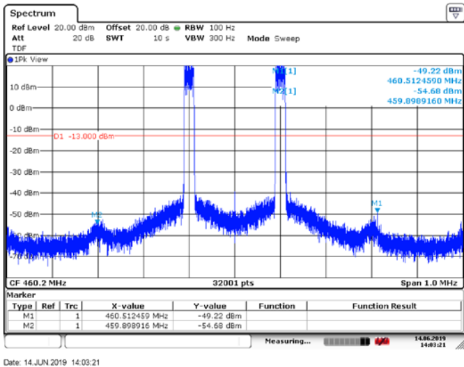
Figure 6.5-48: Conducted Spurious Emissions from inter-modulation products, Tx @low channel of 460 MHz band, 2X7W 25kHzTEDS modulation
