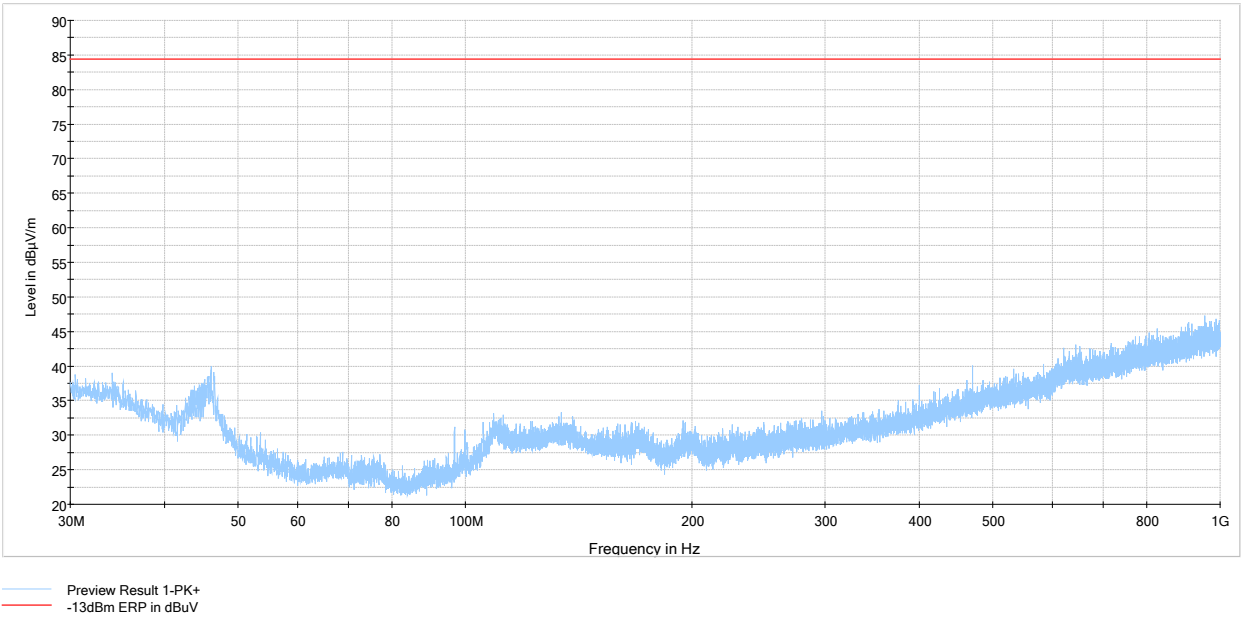
Figure 6.6-27: Cabinet Radiated Spurious Emissions below 1 GHz, Tx @ high channel of 460 MHz band, 50W 16KoF3E modulation
