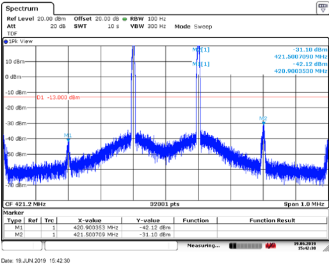
Figure 6.5-37: Conducted Spurious Emissions from inter-modulation products, Tx @low channel of 420 MHz band, 2X15W 7k60FXW modulation
