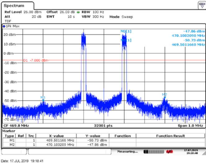
Figure 6.5-52: Conducted Spurious Emissions from inter-modulation products, Tx @ high channel of 460 MHz band, 2X7W 25kHzTEDS modulation
