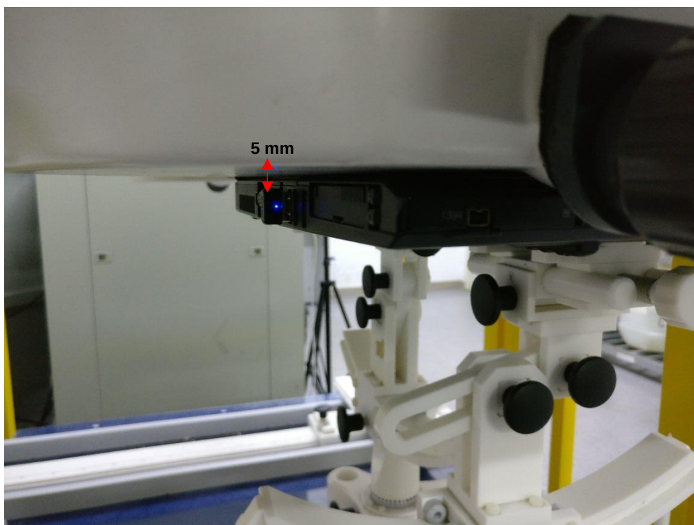
Vertical-Back (5 mm)
