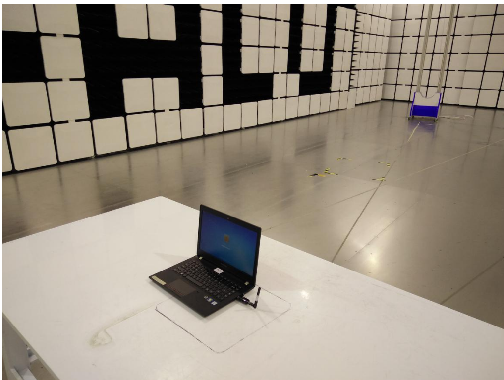
Radiated Test 2
