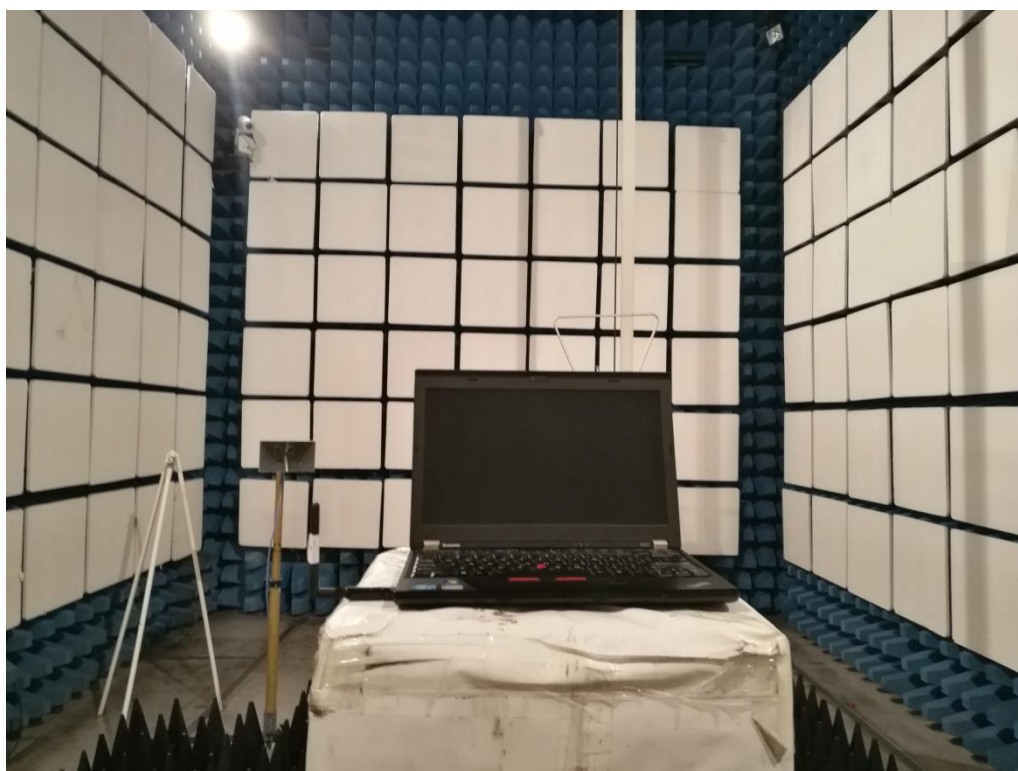
Radiated Test 6
