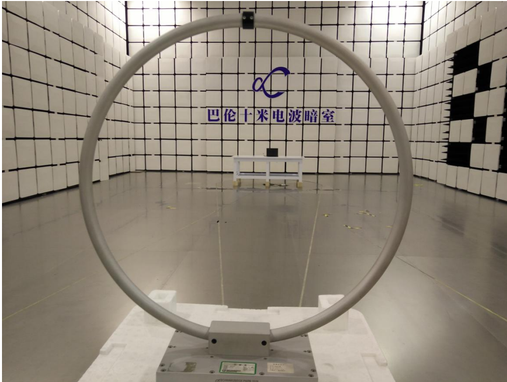
Radiated Test 1
