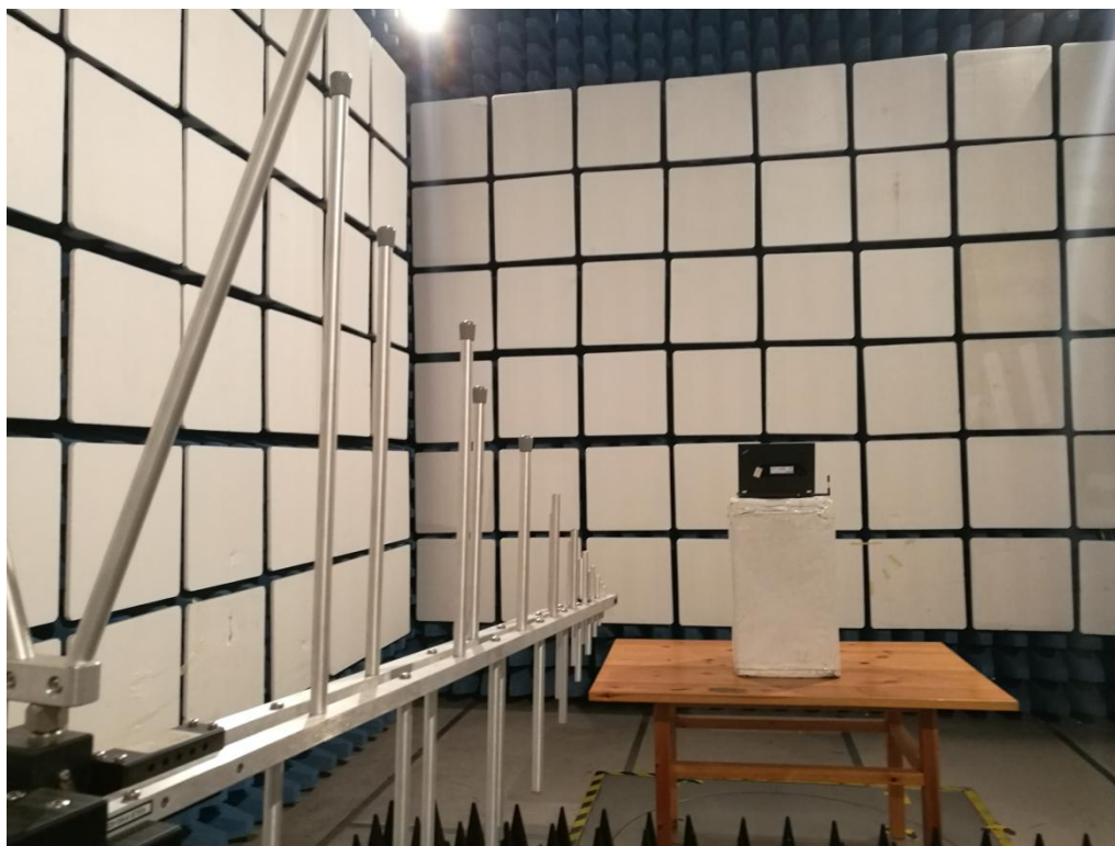
Radiated Test 4
