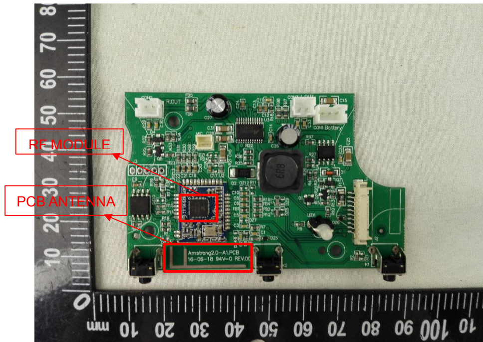
MAIN BOARD TOP VIEW 1
