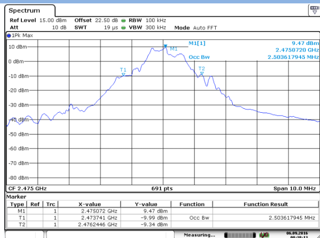
2475 MHz
