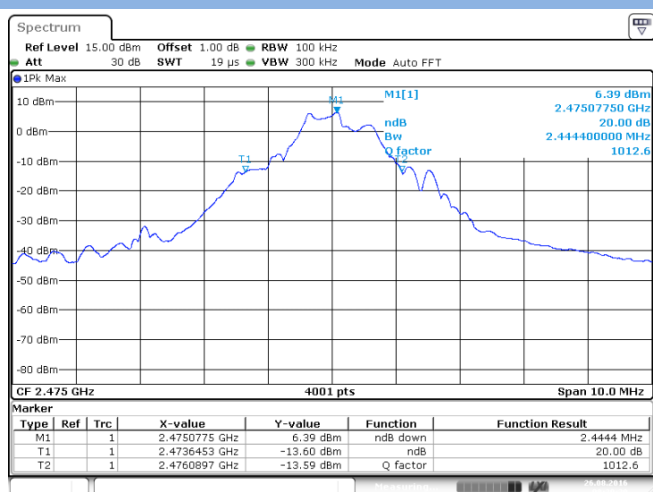
2475 MHz
