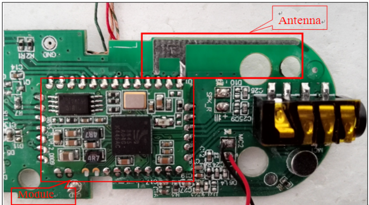
EUT – Module&Antenna View
