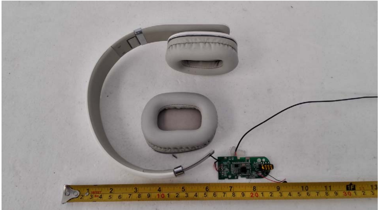
EUT – Cover off View
