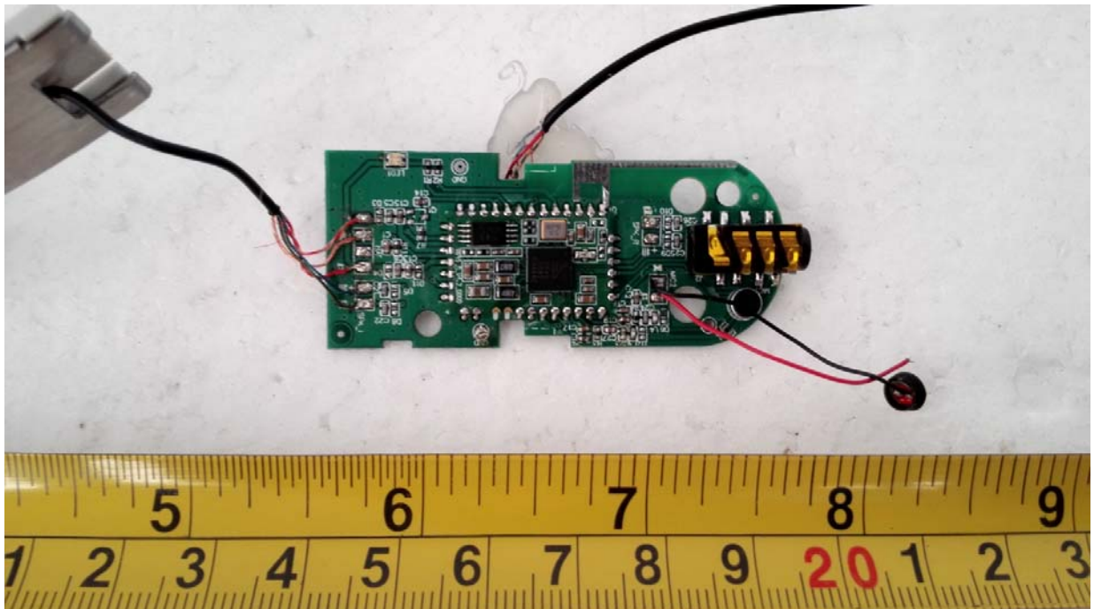
EUT – Mainboard Top View
