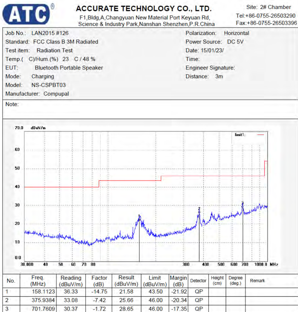
Figure 65: Test figure of Radiated emissions, model NS-CSPBT03, Mode C, Below 1GHz, Horizontal
