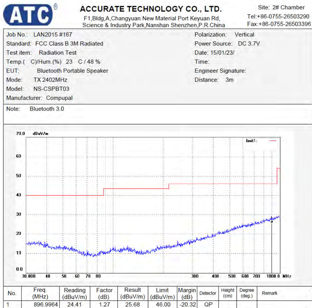
Figure 4: Test figure of spurious emissions, mode A.1, Vertical polarity (30MHz – 1GHz)
