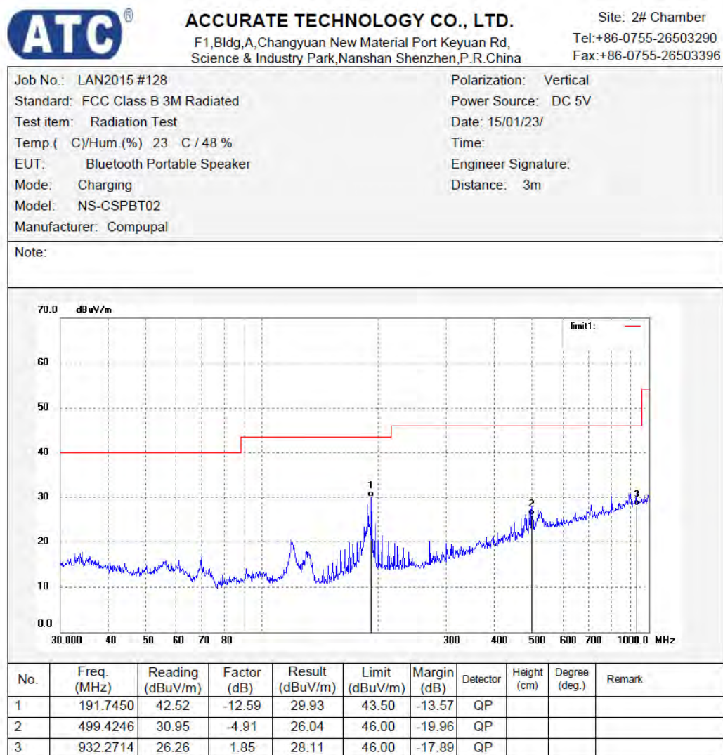
Figure 62: Test figure of Radiated emissions, model NS-CSPBT02, Mode C, Below 1GHz, Vertical
