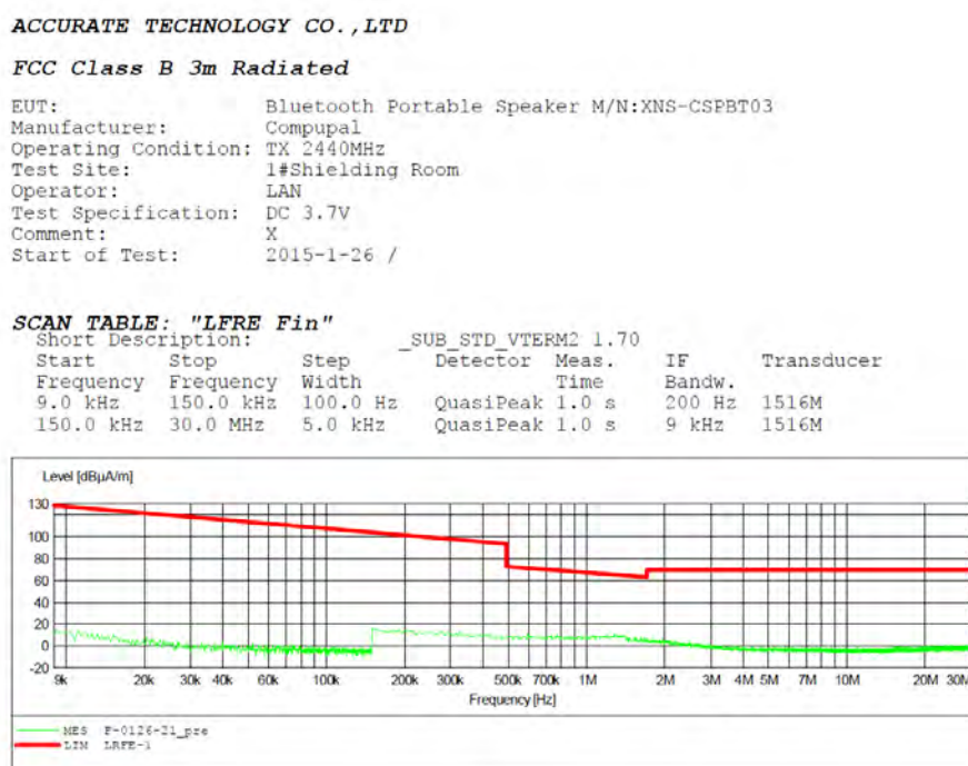
Figure 34: Test figure of spurious emissions, mode B.2, Vertical polarity (9kHz – 30MHz)
