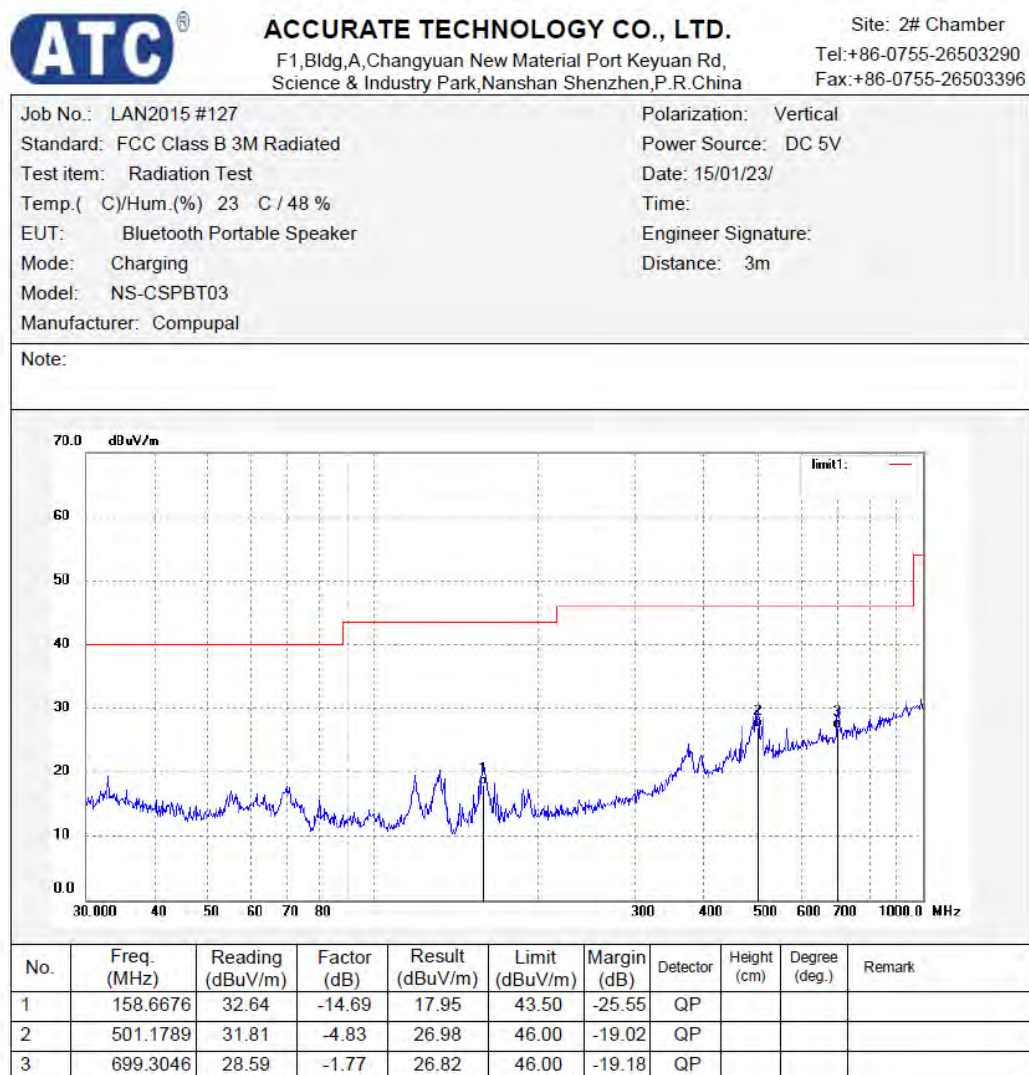
Figure 66: Test figure of Radiated emissions, model NS-CSPBT03, Mode C, Below 1GHz, Vertical
