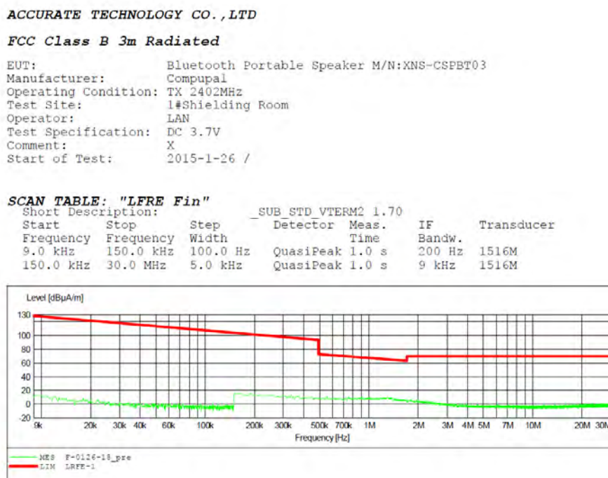
Figure 26: Test figure of spurious emissions, mode B.1, Vertical polarity (9kHz – 30MHz)
