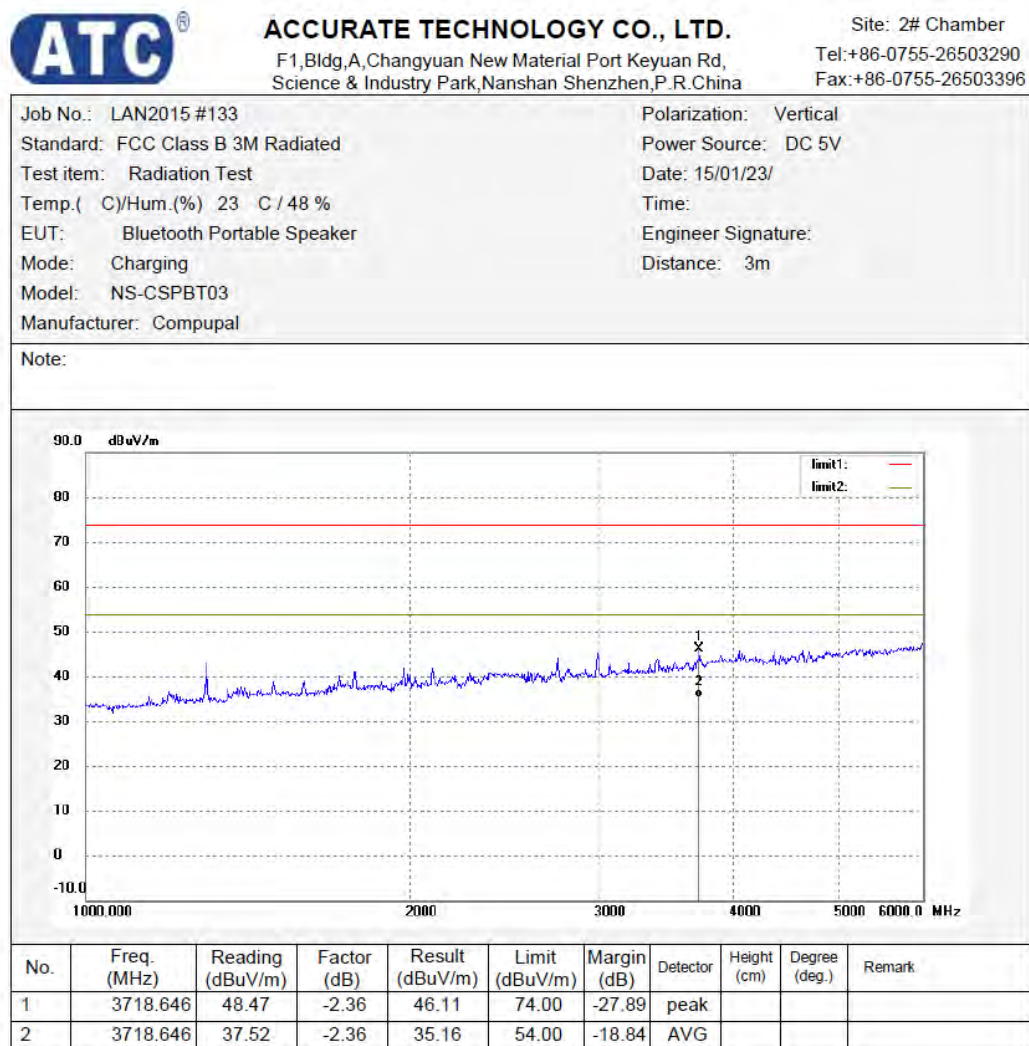
Figure 68: Test figure of Radiated emissions, model NS-CSPBT03, Mode C, Above 1GHz, Vertical
