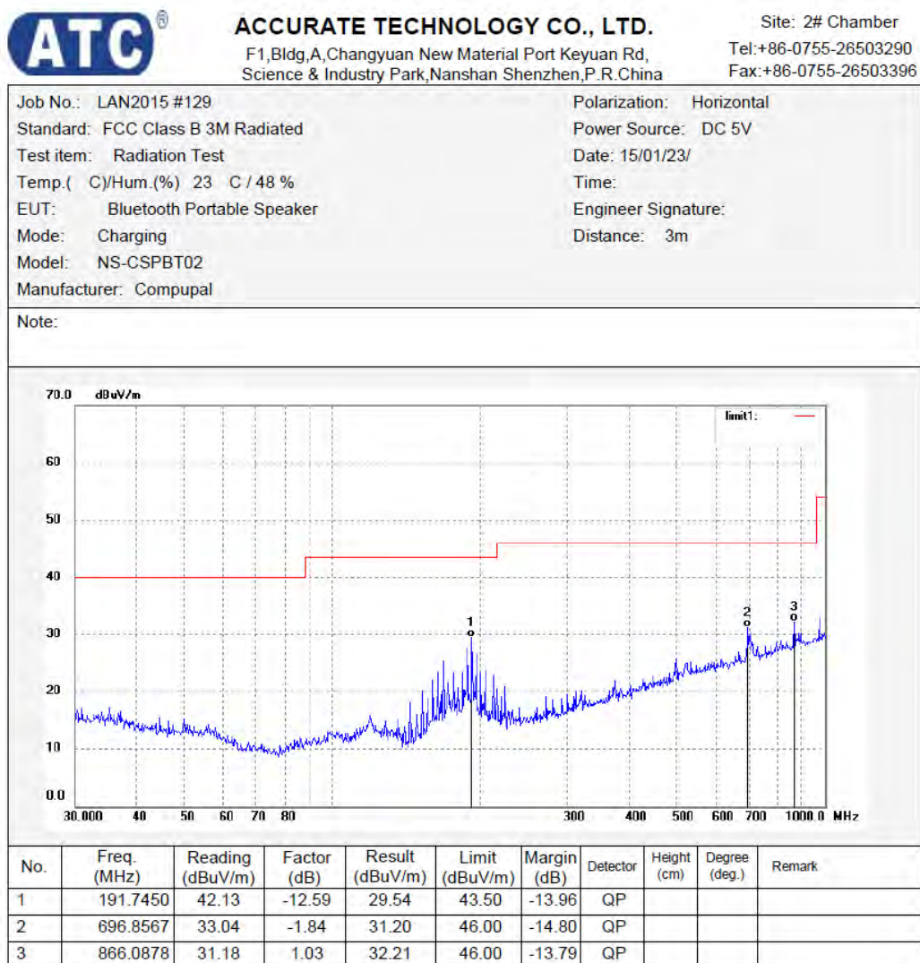
Figure 61: Test figure of Radiated emissions, model NS-CSPBT02, Mode C, Below 1GHz, Horizontal
