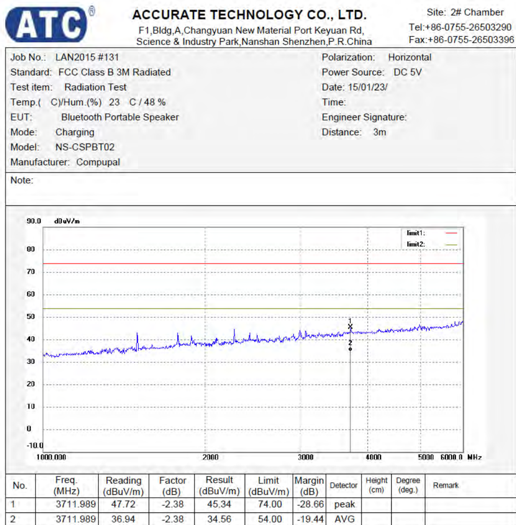
Figure 63: Test figure of Radiated emissions, model NS-CSPBT02, Mode C, Above 1GHz, Horizontal
