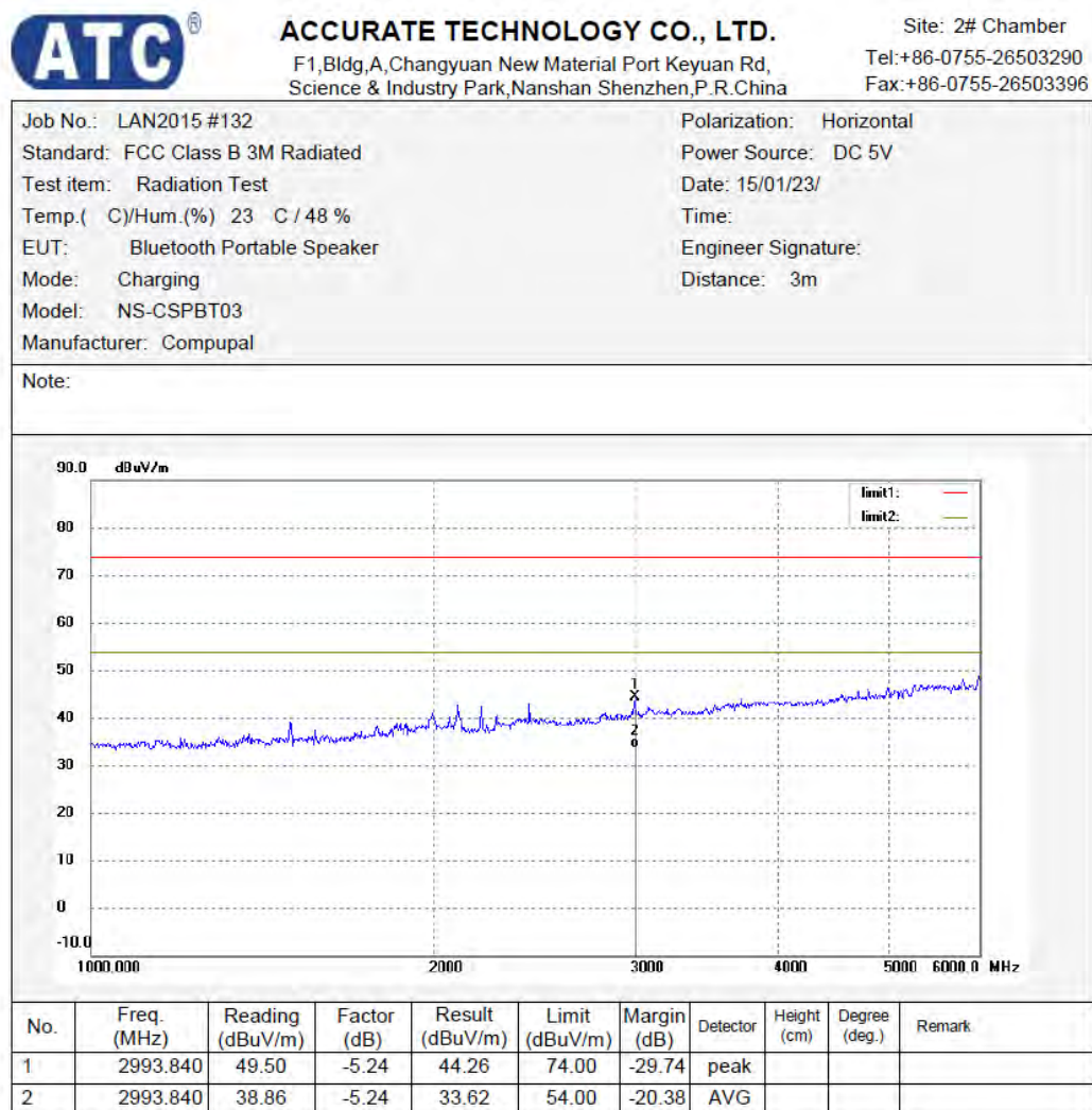
Figure 67: Test figure of Radiated emissions, model NS-CSPBT03, Mode C, Above 1GHz, Horizontal
