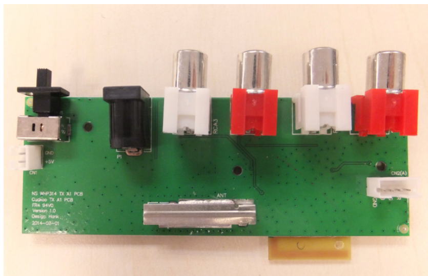
Figure 2 Docking PCB
