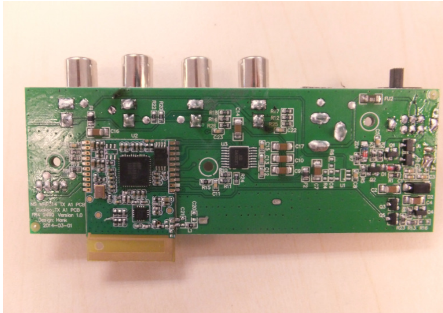
Figure 3 Docking PCB
