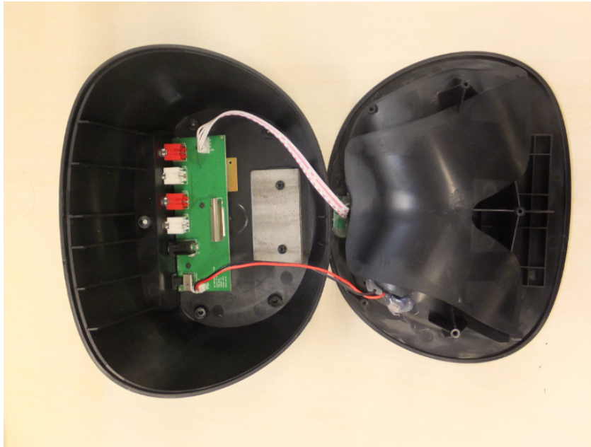
Figure 1 Docking
