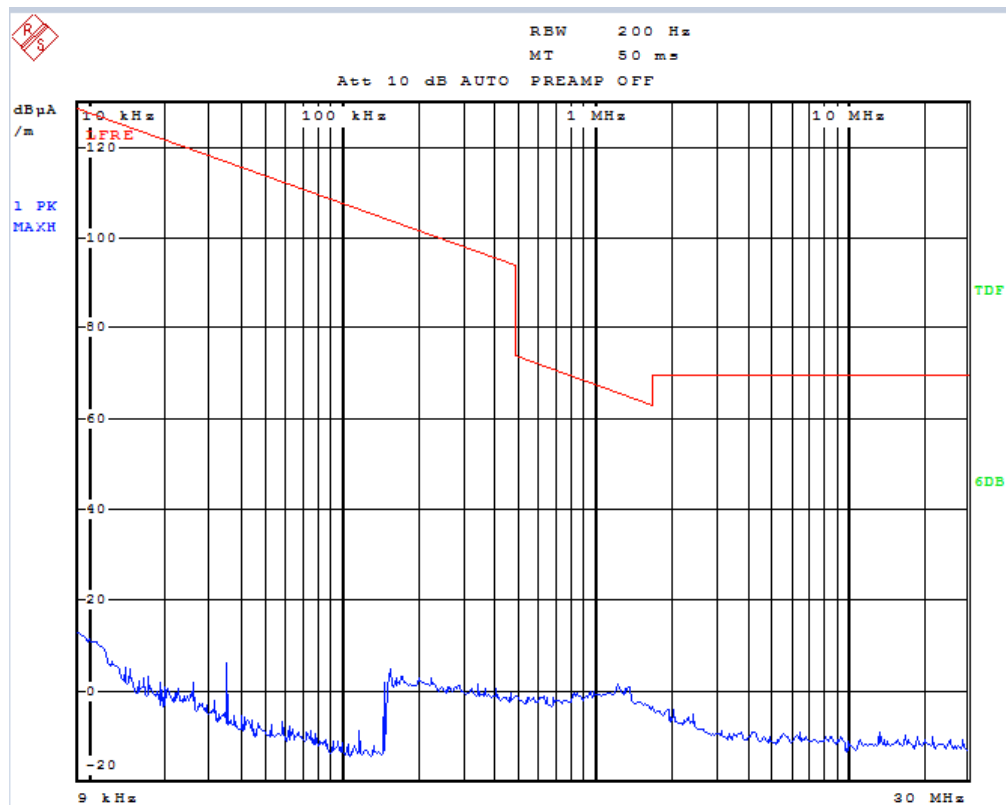
Figure 7: Test figure of radiated spurious emission outside band of docking, high channel, 9 KHz-30MHz, X Axis
