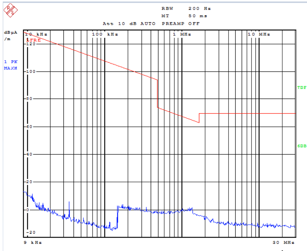
Figure 8: Test figure of radiated spurious emission outside band of docking, high channel, 9 KHz-30MHz, Y Axis
