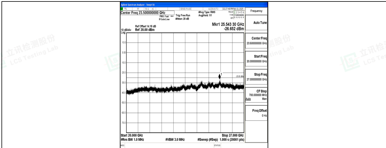
Band7_15MHz_16QAM_20825_1RB#0_20000~27000_20000~27000
