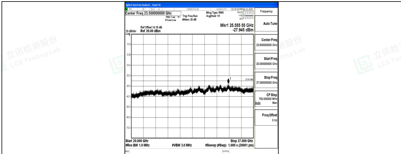
Band7_15MHz_QPSK_21375_1RB#0_20000~27000_20000~27000
