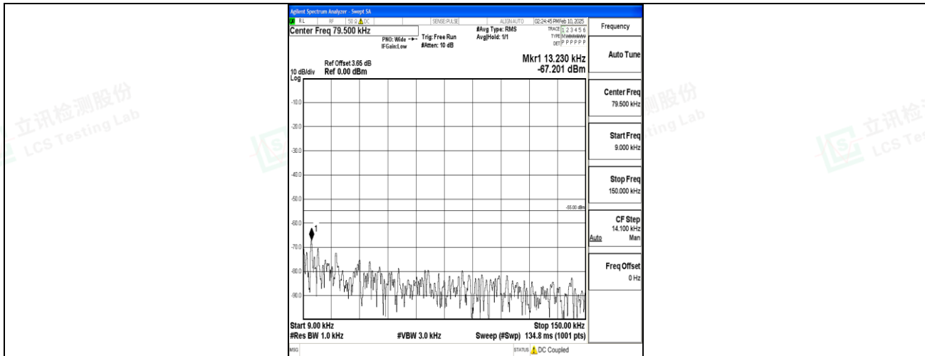
Band7_10MHz_16QAM_21100_1RB#0_0.009~0.15_0.009~0.15
