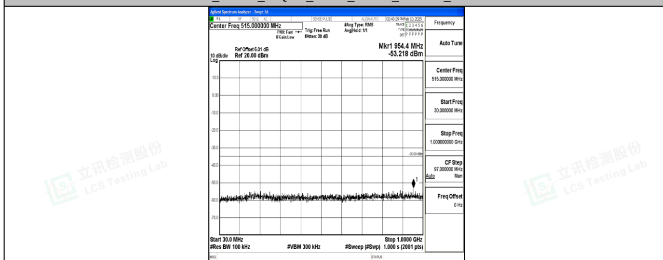
Band7_20MHz_16QAM_20850_1RB#0_30~1000_30~1000
