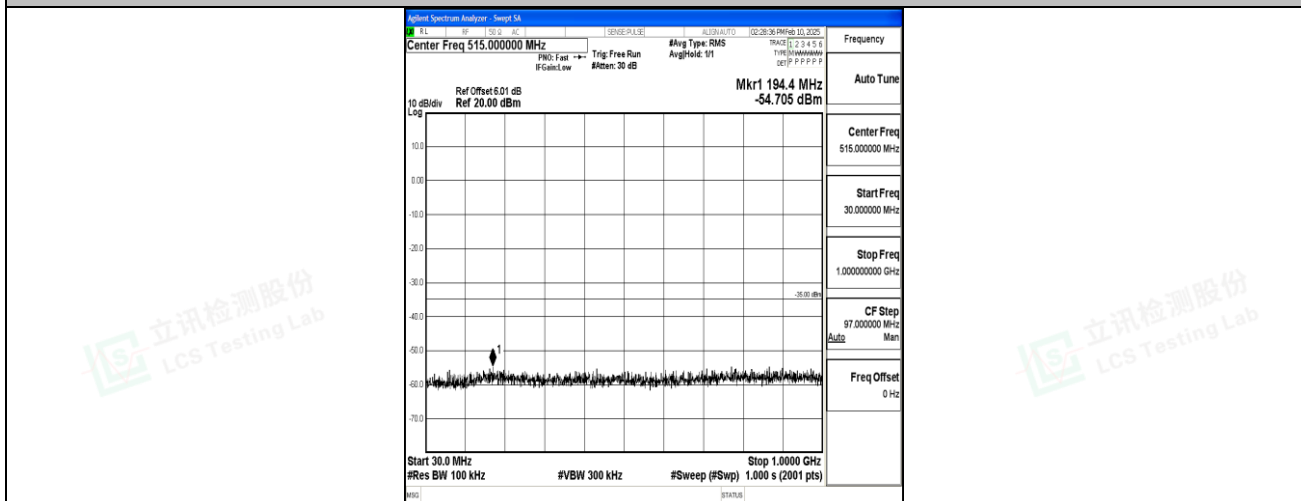
Band7_15MHz_16QAM_21100_1RB#0_30~1000_30~1000
