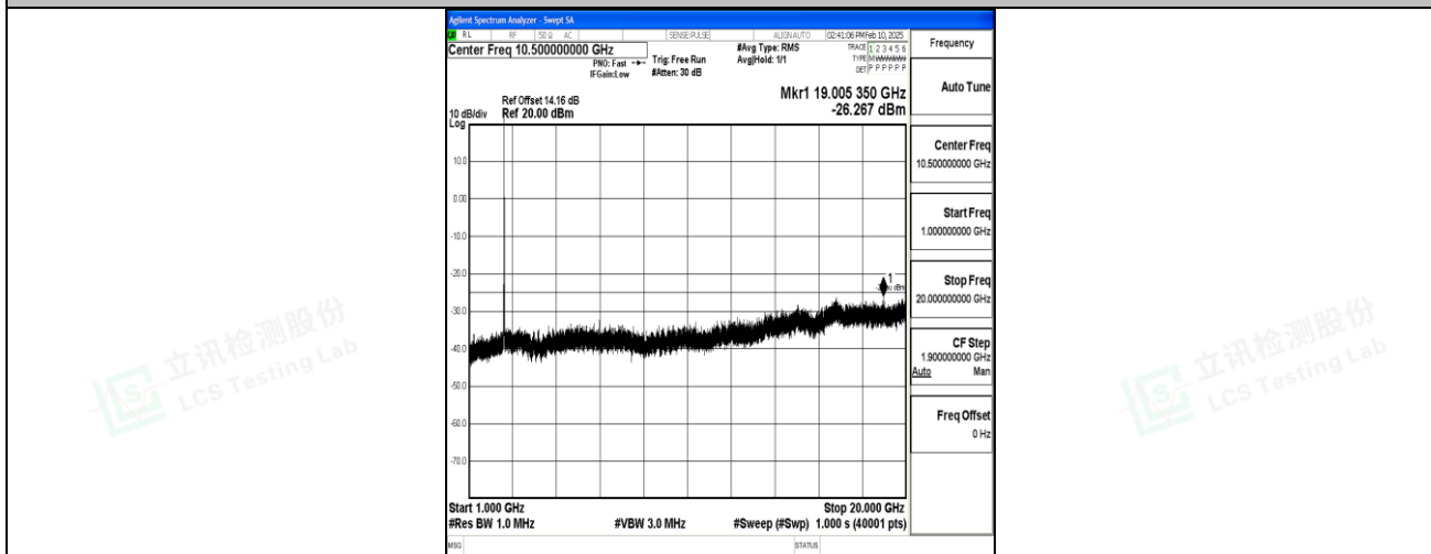
Band7_20MHz_QPSK_21100_1RB#0_1000~20000_1000~20000
