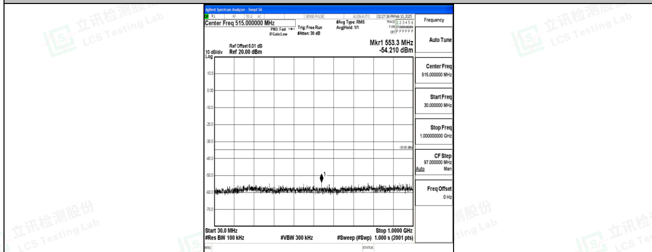
Band7_15MHz_16QAM_20825_1RB#0_30~1000_30~1000
