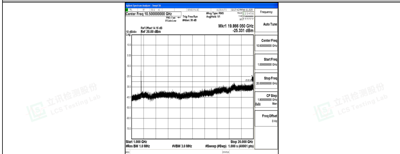
Band7_15MHz_16QAM_20825_1RB#0_1000~20000_1000~20000
