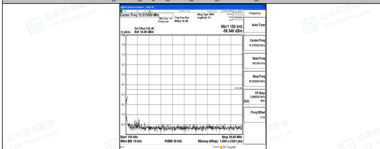
Band7_20MHz_16QAM_20850_1RB#0_0.15~30_0.15~30
