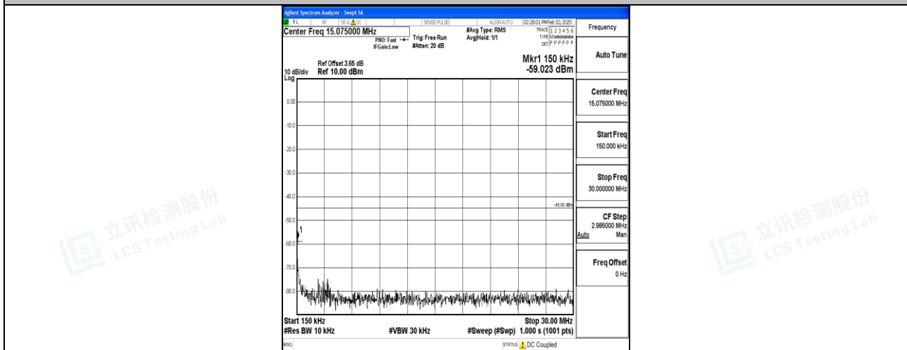
Band7_15MHz_QPSK_21100_1RB#0_0.15~30_0.15~30
