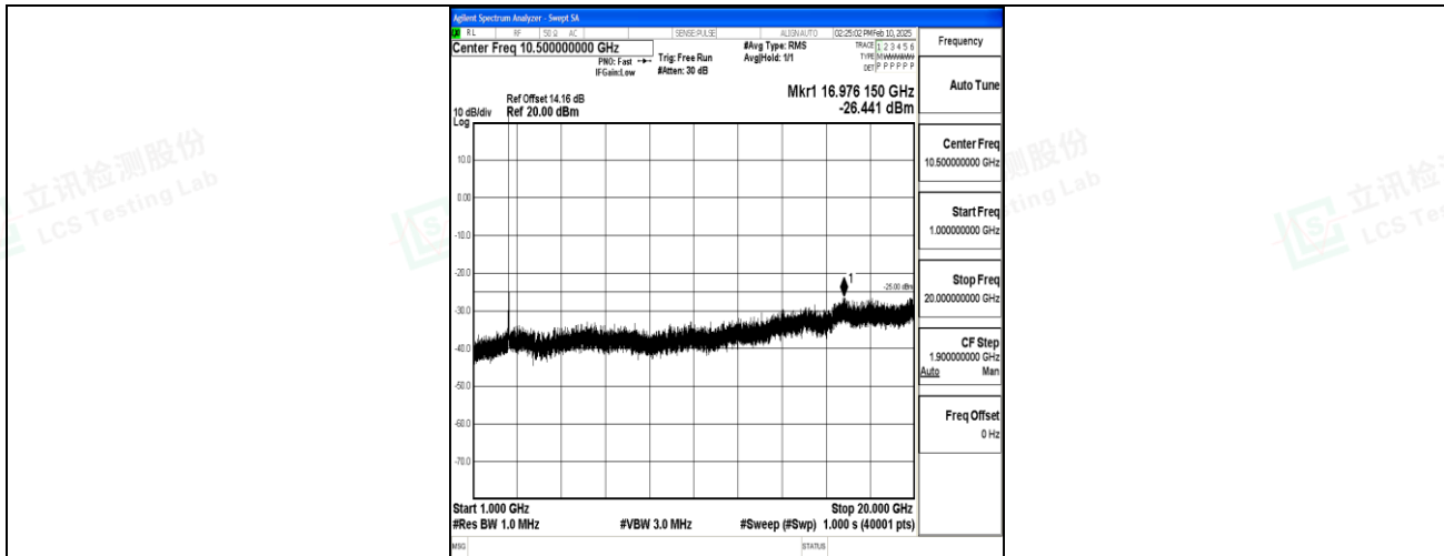
Band7_10MHz_16QAM_21100_1RB#0_1000~20000_1000~20000
