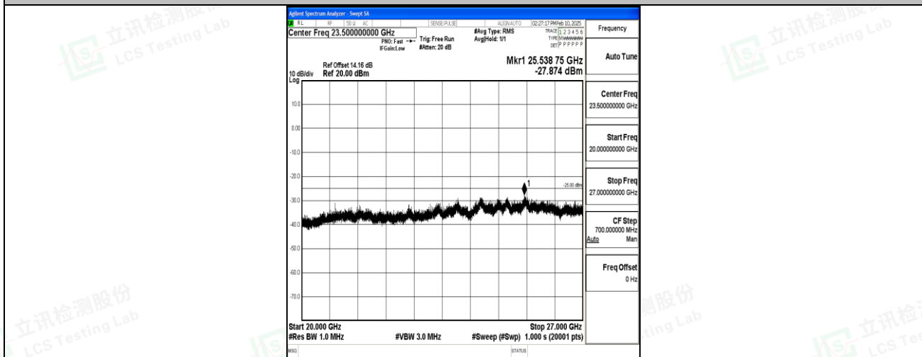
Band7_15MHz_QPSK_20825_1RB#0_20000~27000_20000~27000
