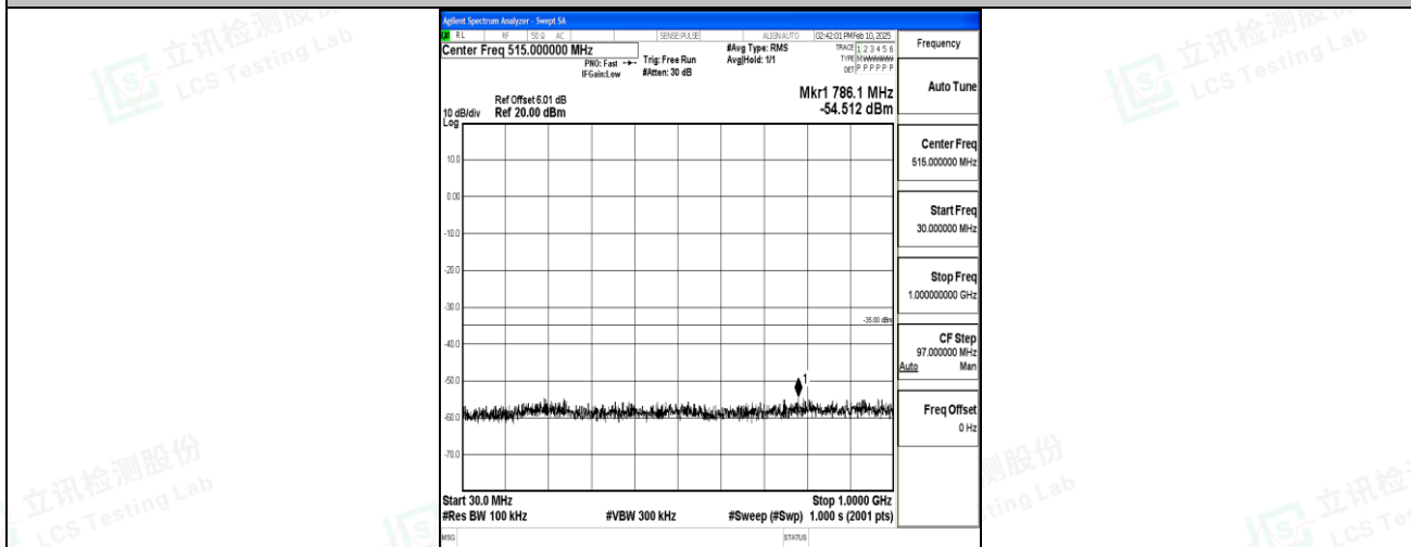
Band7_20MHz_QPSK_21350_1RB#0_30~1000_30~1000
