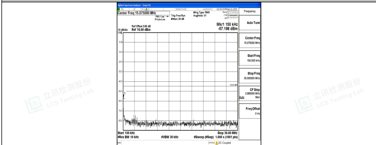
Band7_15MHz_16QAM_21375_1RB#0_0.15~30_0.15~30
