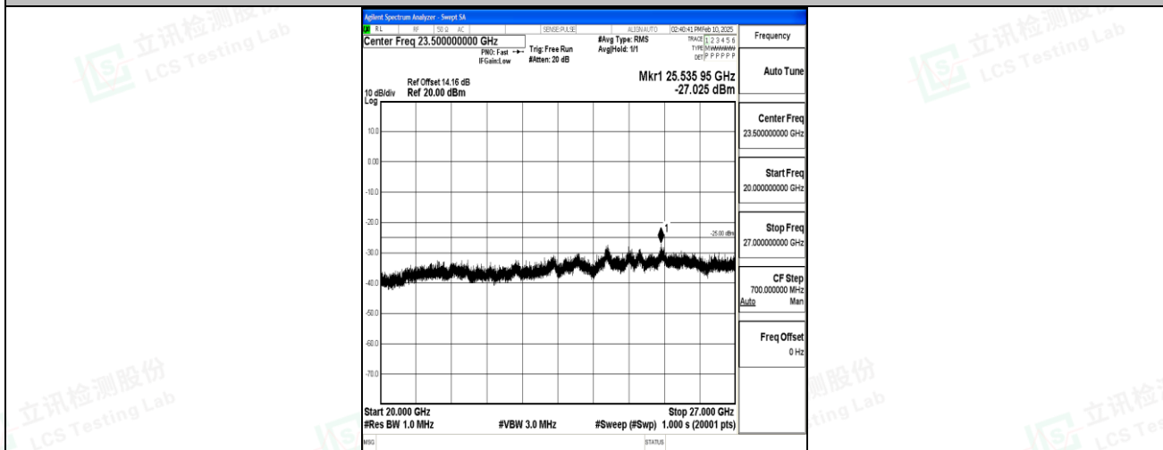
Band7_20MHz_16QAM_20850_1RB#0_20000~27000_20000~27000
