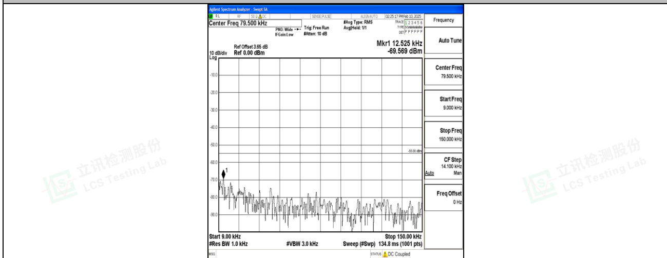
Band7_10MHz_QPSK_21400_1RB#0_0.009~0.15_0.009~0.15
