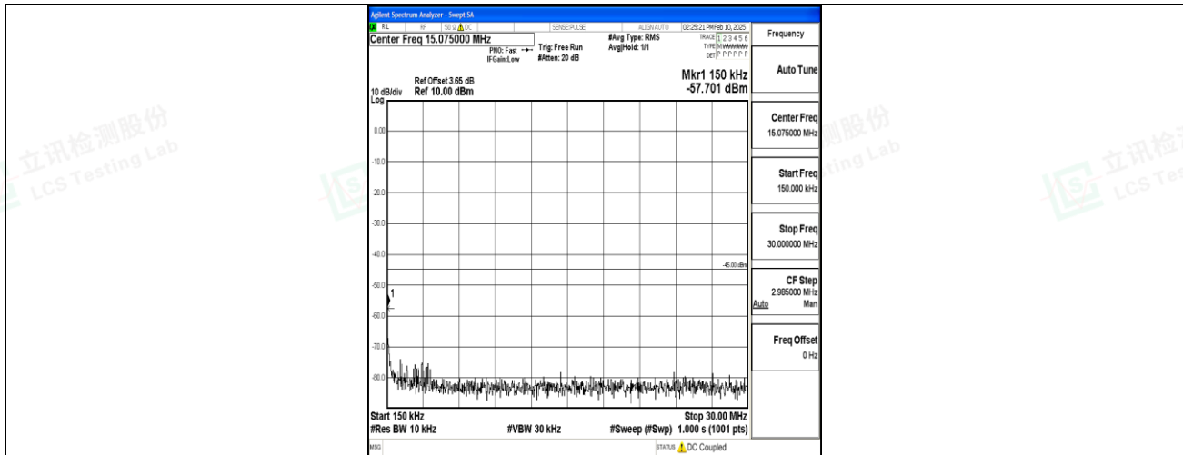
Band7_10MHz_QPSK_21400_1RB#0_0.15~30_0.15~30
