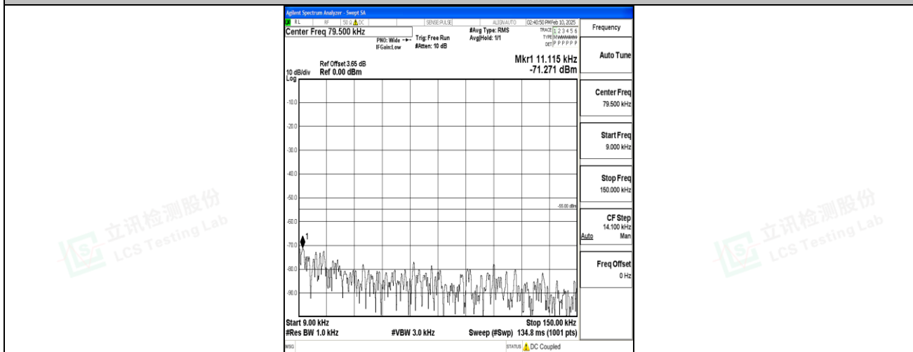
Band7_20MHz_QPSK_21100_1RB#0_0.009~0.15_0.009~0.15
