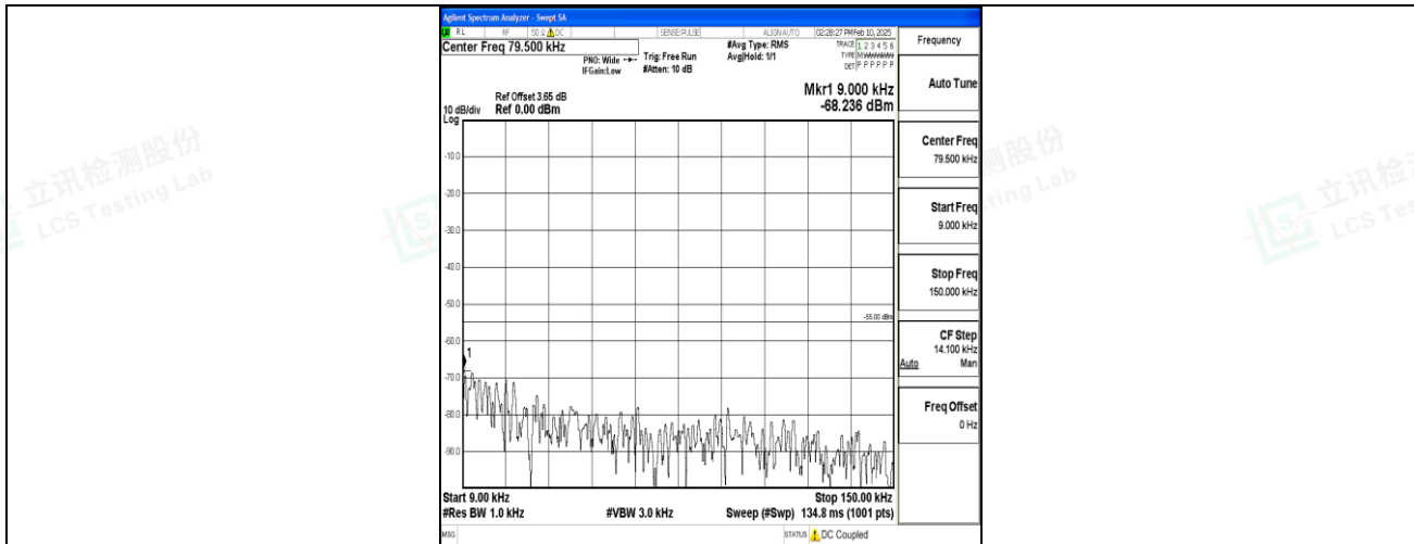
Band7_15MHz_16QAM_21100_1RB#0_0.009~0.15_0.009~0.15
