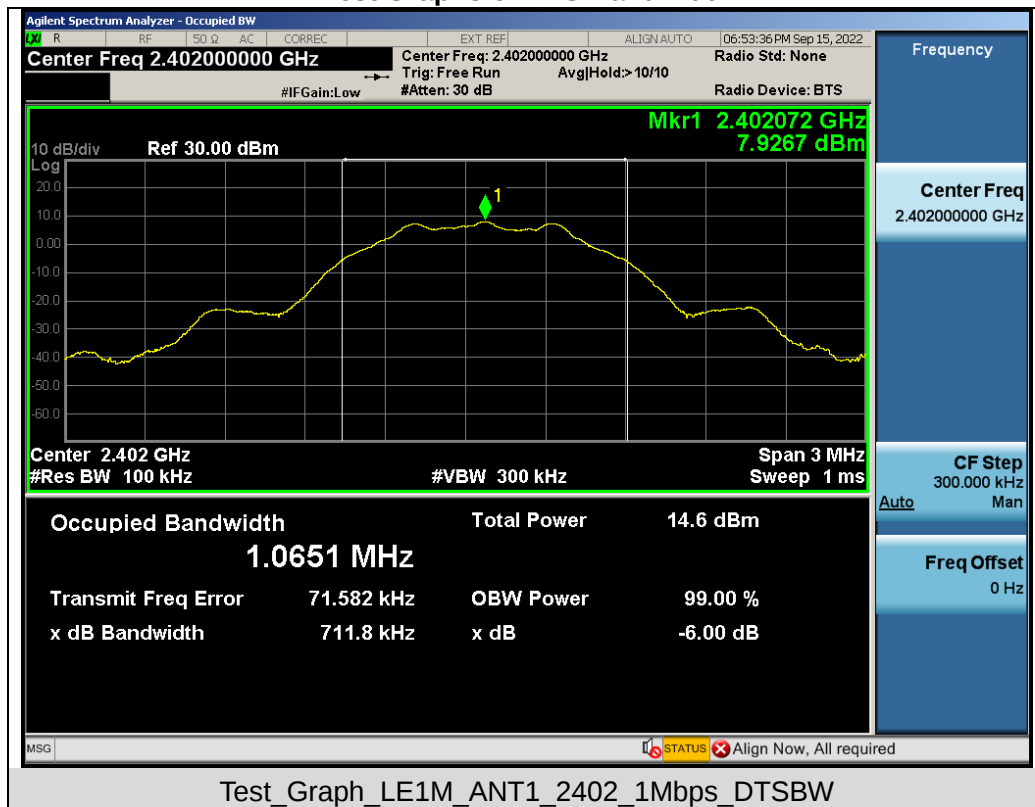
1M Test Graphs of DTS Bandwidth
