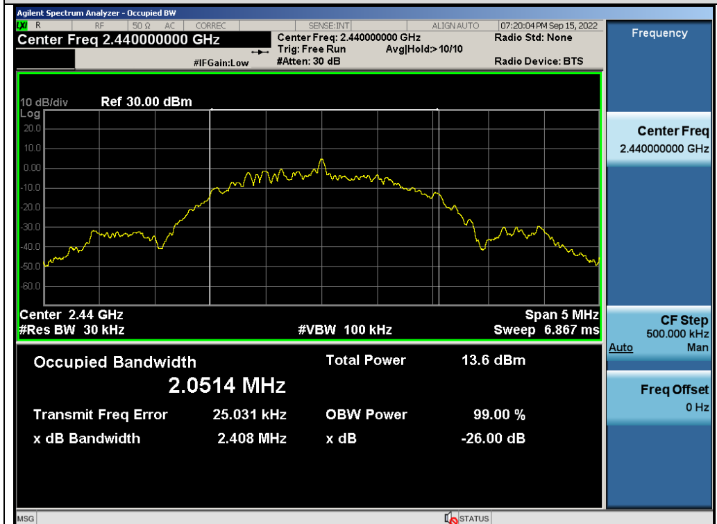
Test_Graph_LE2M_ANT1_2440_2Mbps_OBW
