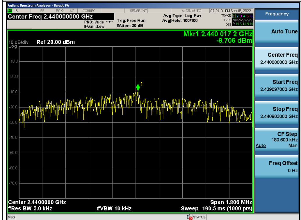
Test_Graph_LE2M_ANT1_2440_2Mbps_PSD
