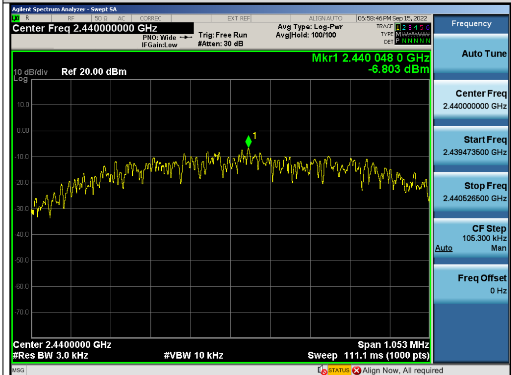
Test_Graph_LE1M_ANT1_2440_1Mbps_PSD
