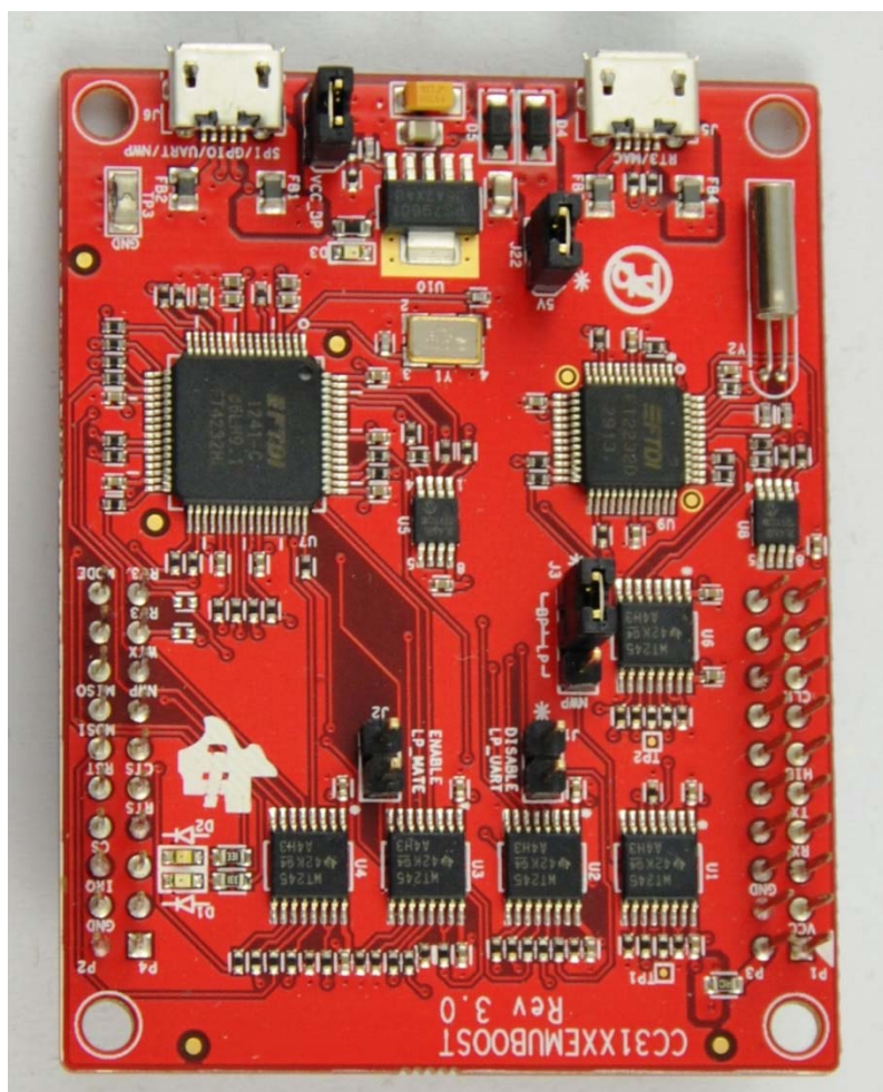
Figure 7-6: CC31XXEMUBOOST board
