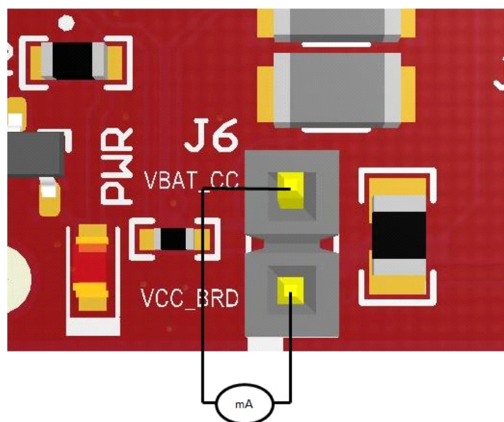
Figure 7-4: Low-Current Measurement
