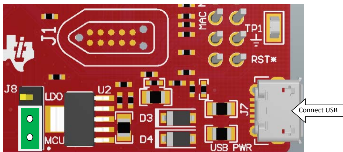
Figure 7-9: Jumper Configuration when working with Launchpad kit
