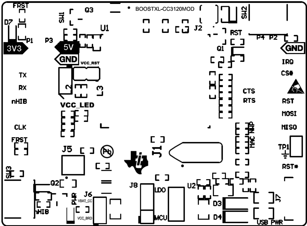
Figure 1-4: BOOSTXL-CC3120MOD Top Overlay
