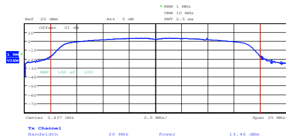
Figure 8.4-3: Output power on 802.11n, sample plot
