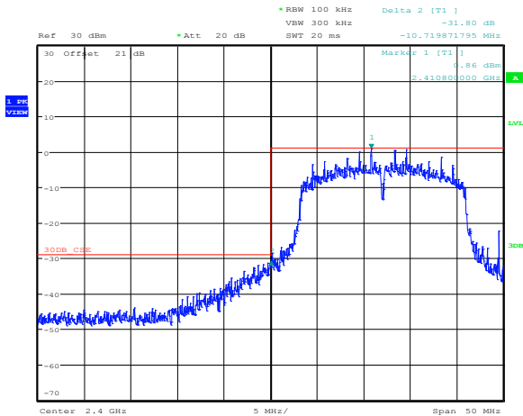
Figure 8.5-13: Conducted outside restricted bands band edge emissions for 802.11b, at 2.4 GHz
