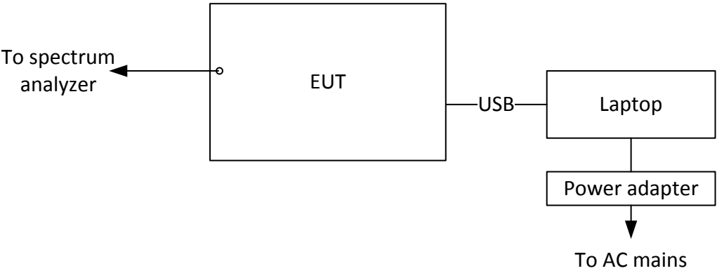
Figure 3.6-1: Setup diagram
