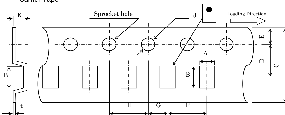
Dimensions (mm)
