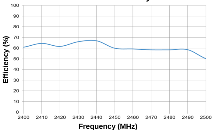
2.4 GHz Efficiency
