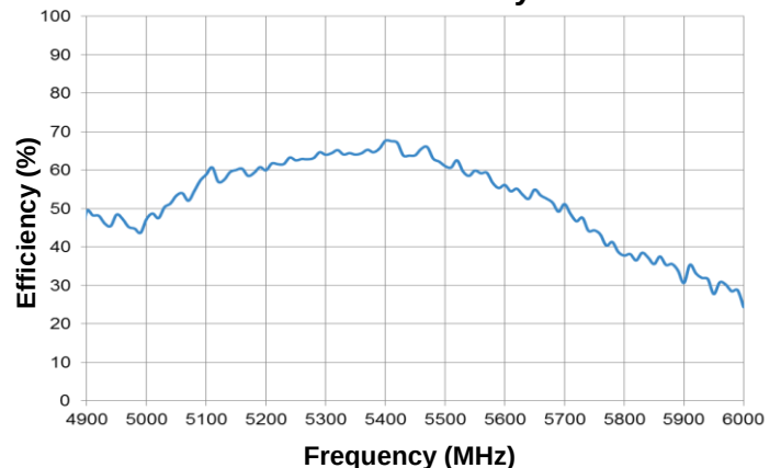
5 GHz Efficiency
