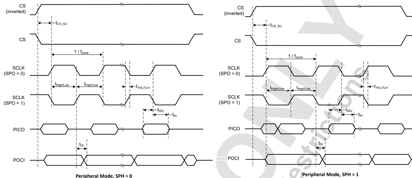
Figure 6-5. SPI Timing
