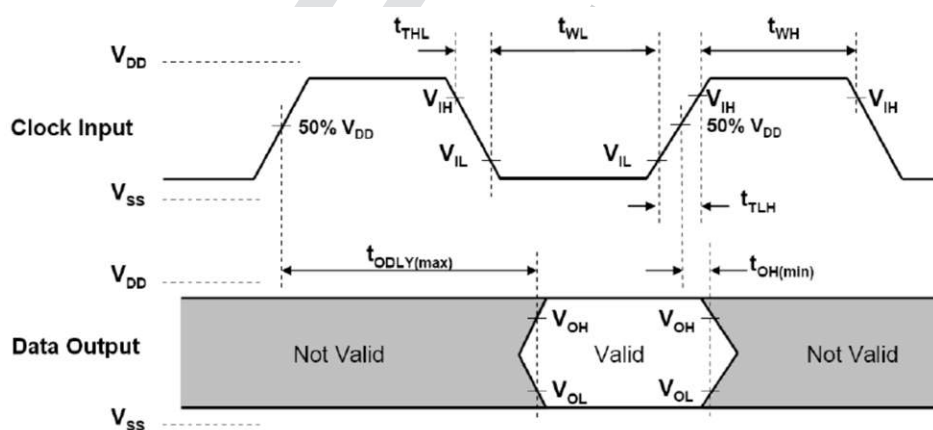
Figure 6-4. SDIO HS Output Timing
