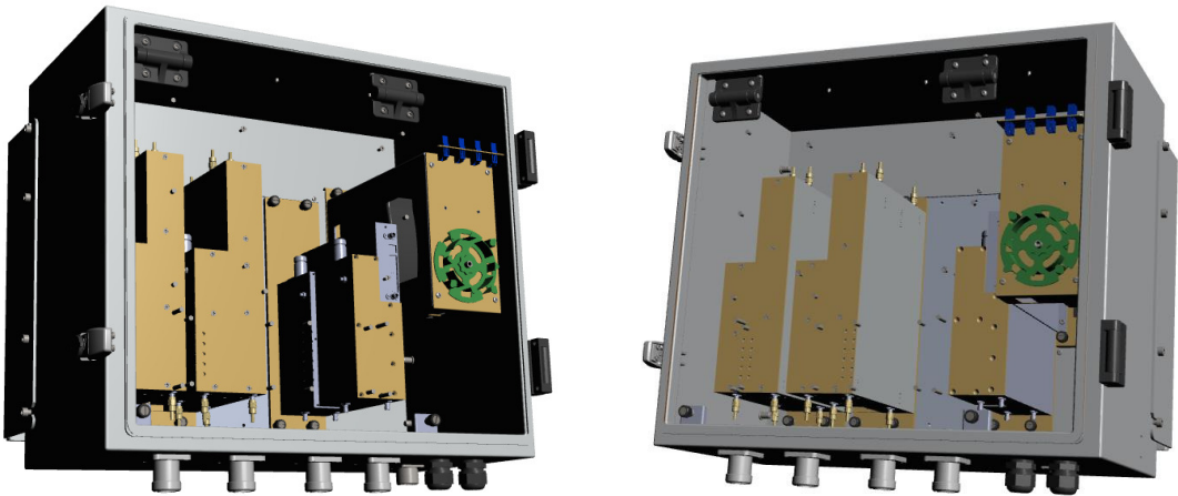
Figure 2-6 RHU Inside drawing
