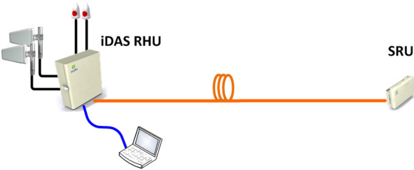
Figure 4-2 RHU-SRU network
