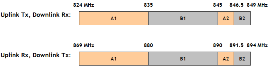
Figure 2-9 Frequency allocation of 850 MHz band
