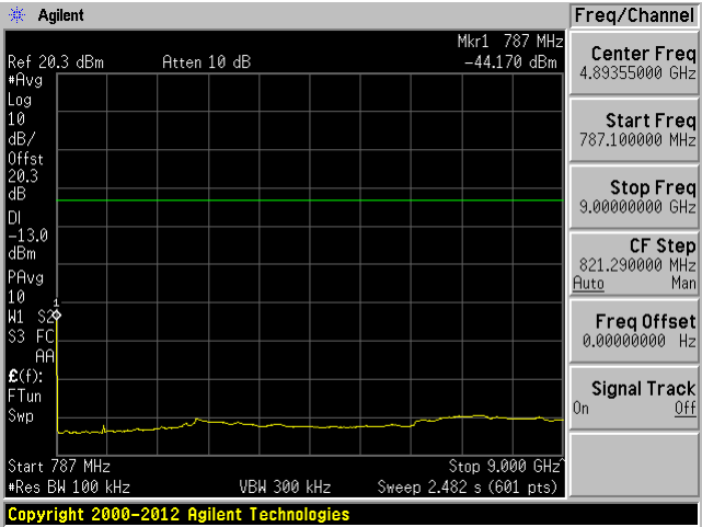
Low Channel: 787.1 MHz-9 GHz
