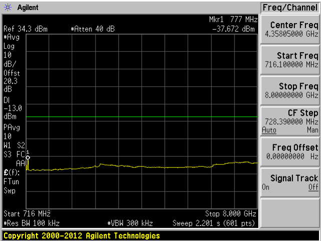
Middle Channel: 716.1 MHz-8 GHz
