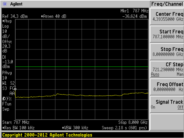
Low Channel: 787.1 MHz-8 GHz
