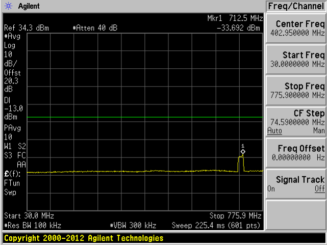
High Channel: 30 MHz-775.9 MHz
