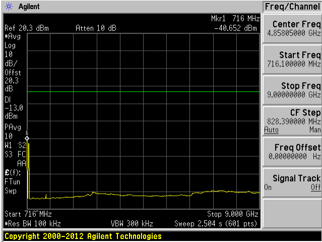
Low Channel: 716.1 MHz- 9 GHz
