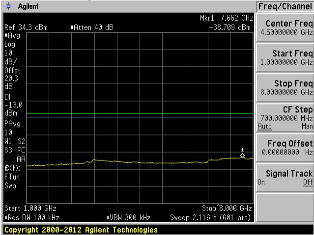
High Channel: 1 GHz- 8 GHz
