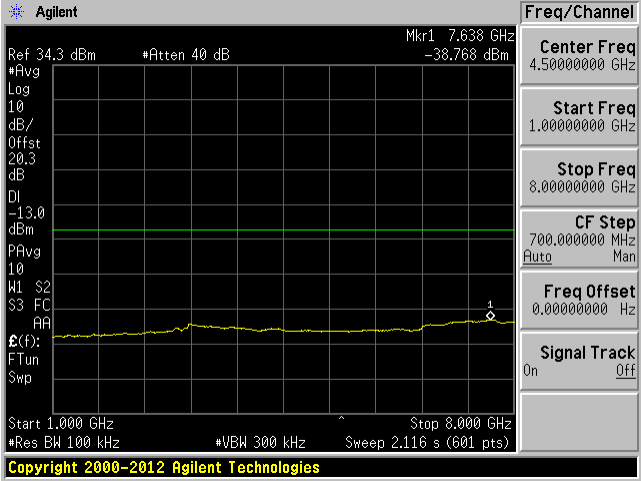
Middle Channel: 1 GHz- 8 GHz
