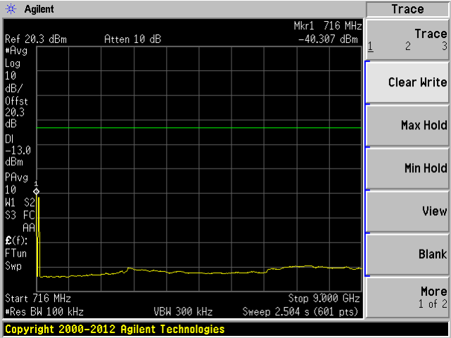
Middle Channel: 716.1 MHz-9 GHz
