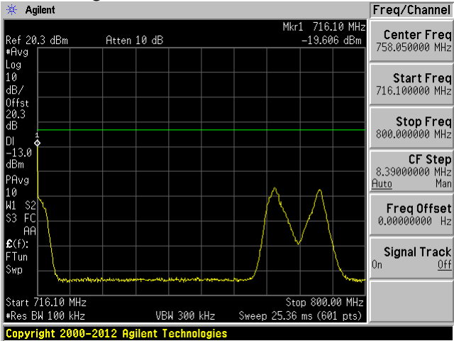
High Channel: 716.1 MHz-800 MHz
