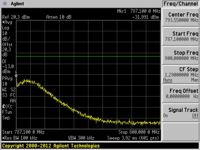
High Channel: 787.1 MHz-800 MHz
