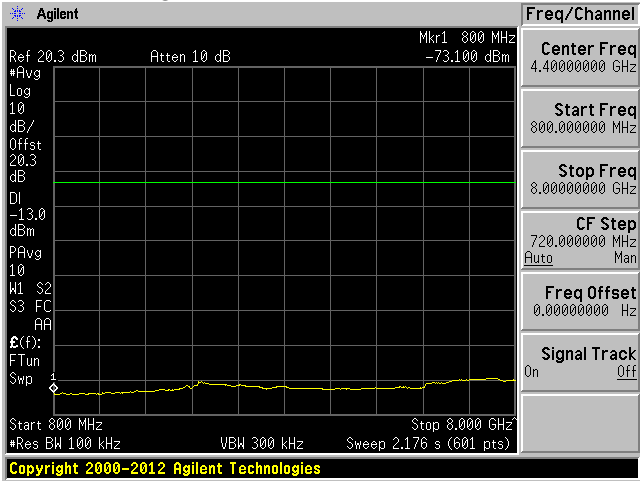
High Channel: 800 MHz- 8 GHz
