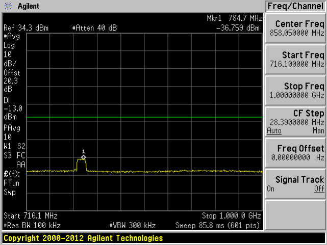
High Channel: 716.1 MHz-1 GHz
