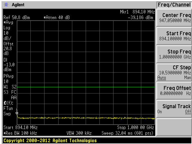
High Channels: 894.1 MHz-1 GHz
