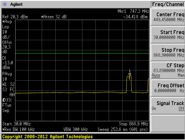
Middle Channel: 30 MHz-868.9 MHz
