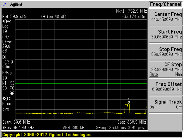
High Channel: 30 MHz-868.9 MHz
