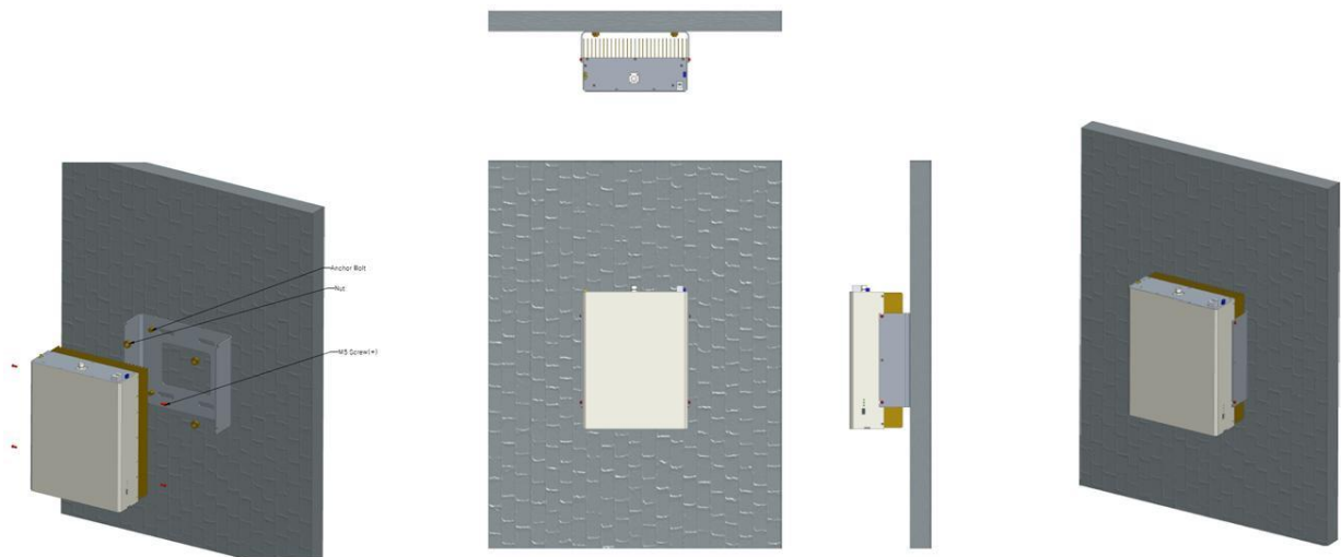
Figure 3-1 Wall mounting
