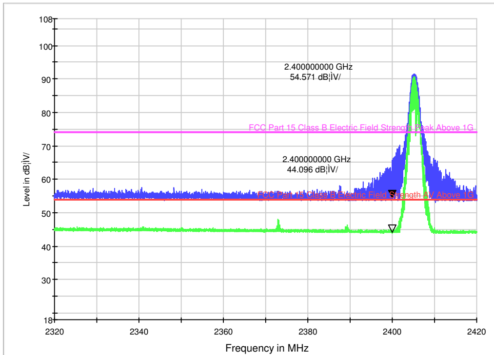
Electric Field Strength 1-18GdBuV TX
