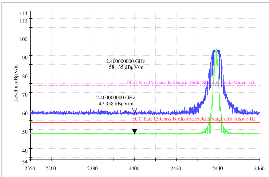
Electric Field Strength 1-18GdBuV TX EIRP
