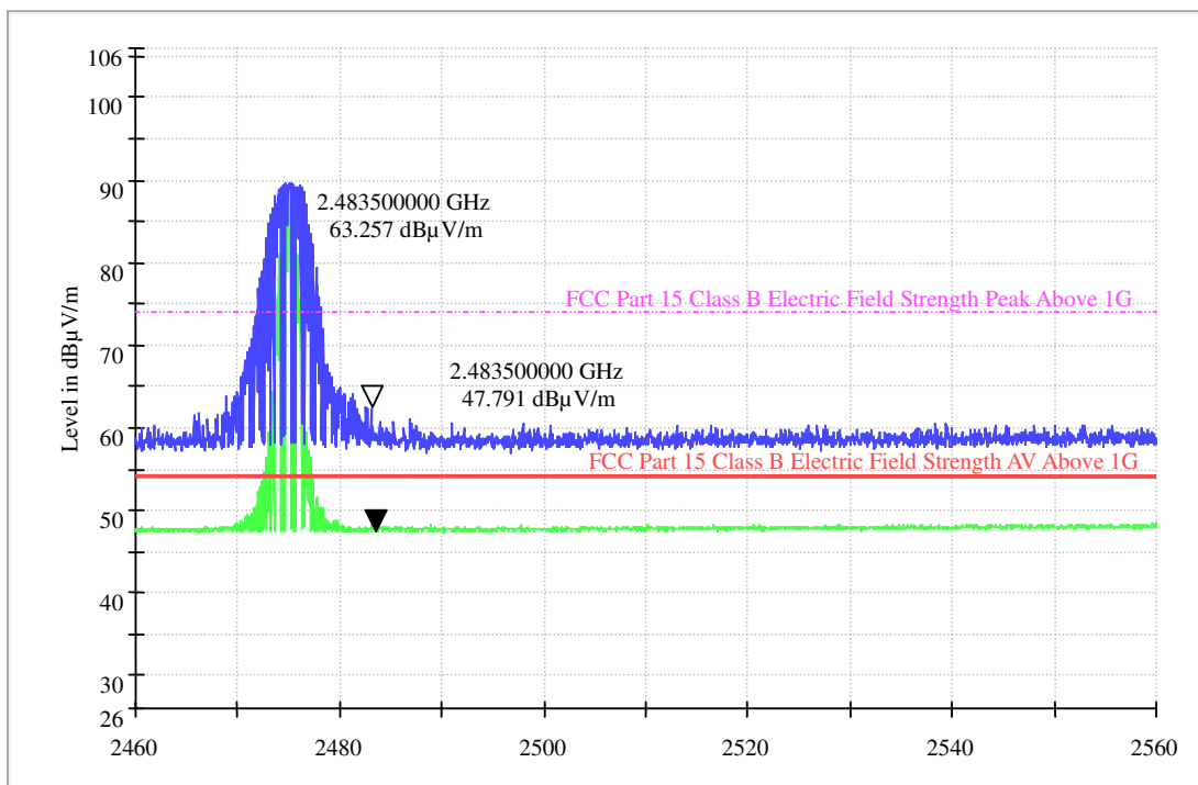
Electric Field Strength 1-18GdBuV TX EIRP
