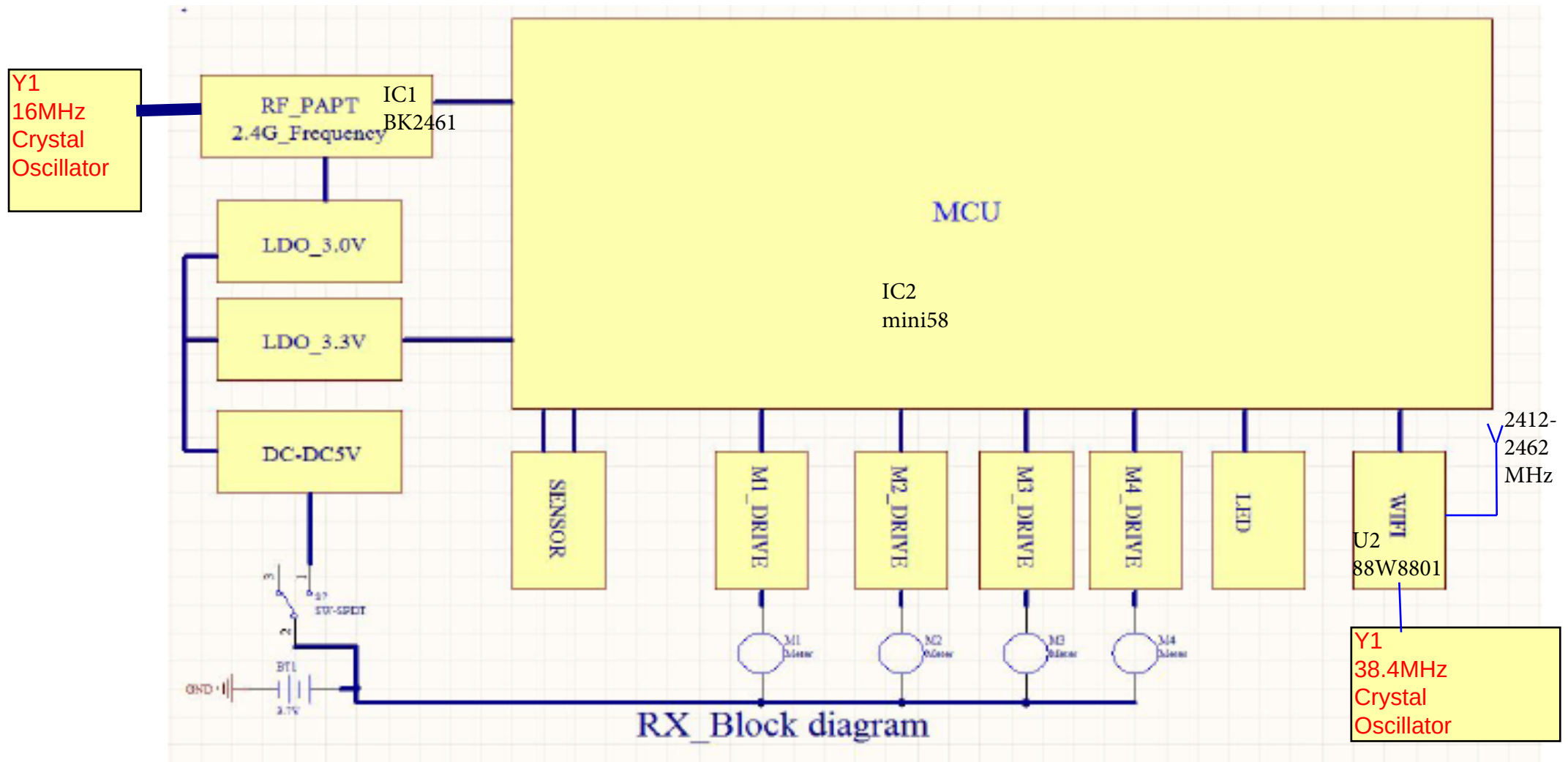
RX_Block diagram
