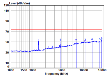
11ax_20M_TX_CH_01_Vertical
