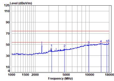
11ax_20M_TX_CH_06_Vertical
