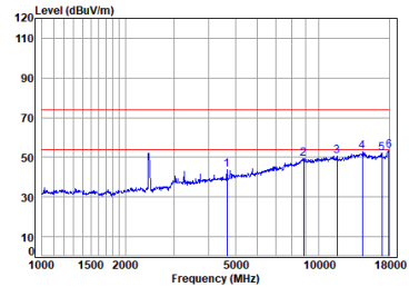
11ax_40M_TX_CH_06_Vertical
