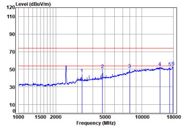
11ax_40M_TX_CH_03_Vertical
