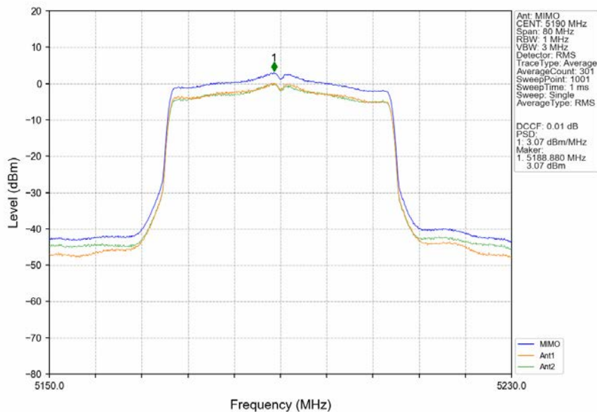
802.11ax(HEW40)_LCH_5190MHz_RU484_Left_MIMO_NTNV
