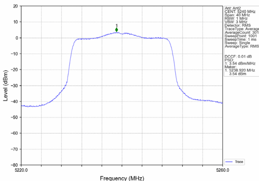
802.11ax(HEW20)_HCH_5240MHz_RU242_Left_MIMO_NTNV
