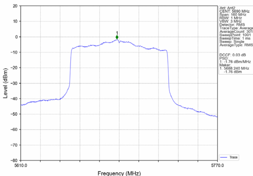
802.11ax(HEW80)_HCH_5690MHz_RU996_Left_MIMO_NTNV
