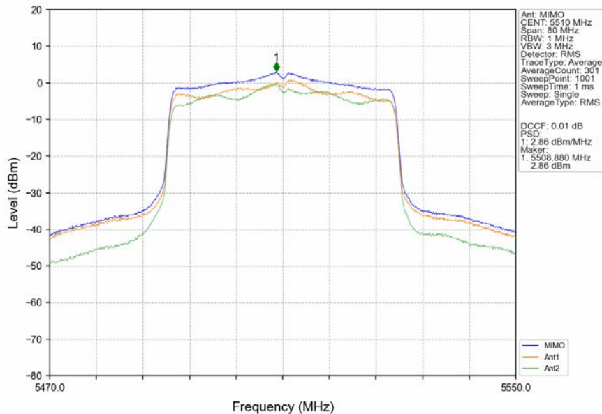
802.11ax(HEW40)_LCH_5510MHz_RU484_Left_MIMO_NTNV
