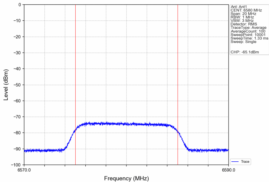
802.11ax(HEW160)_HCH_6505MHz_Inject signal_6580MHz_Detection status_Minimal
