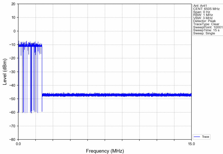
802.11ax(HEW160)_HCH_6505MHz_Inject signal_6505MHz_OFF
