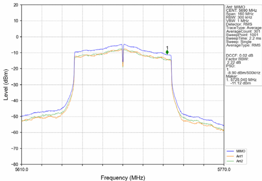
802.11ac(VHT80)_HCH_5690MHz_MIMO_NTNV
