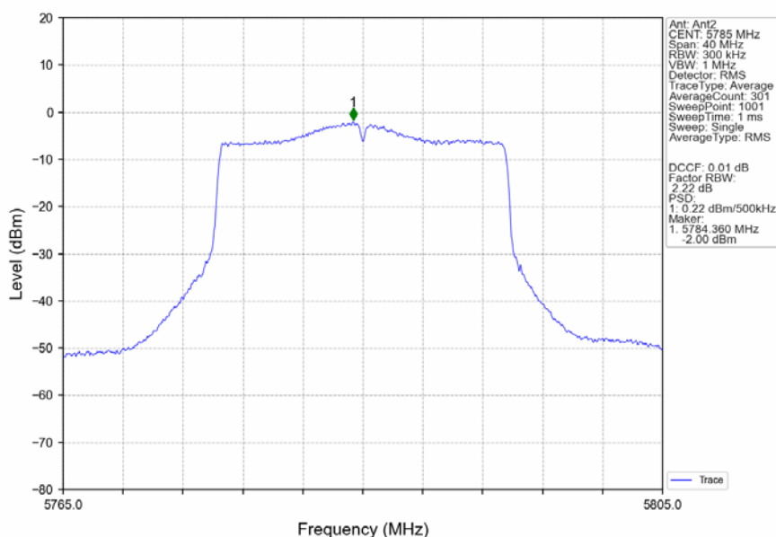
802.11ax(HEW20)_MCH_5785MHz_RU242_Left_MIMO_NTNV
