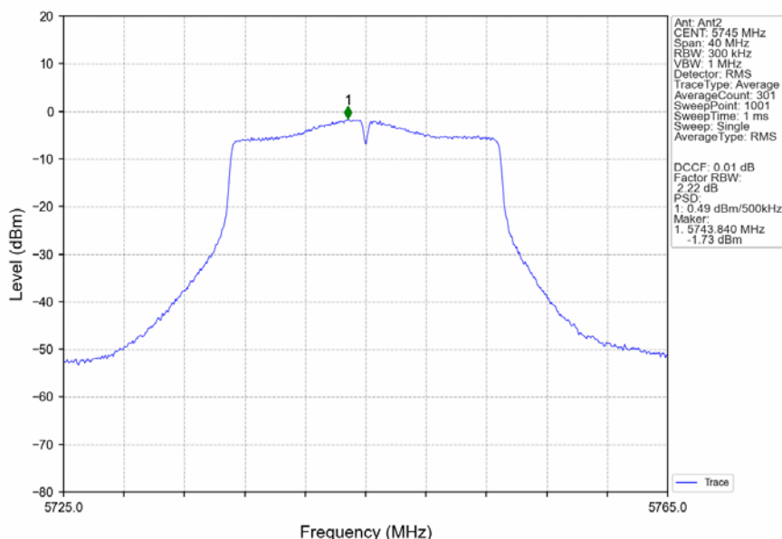
802.11n(HT20)_LCH_5745MHz_Ant2_NTNV
