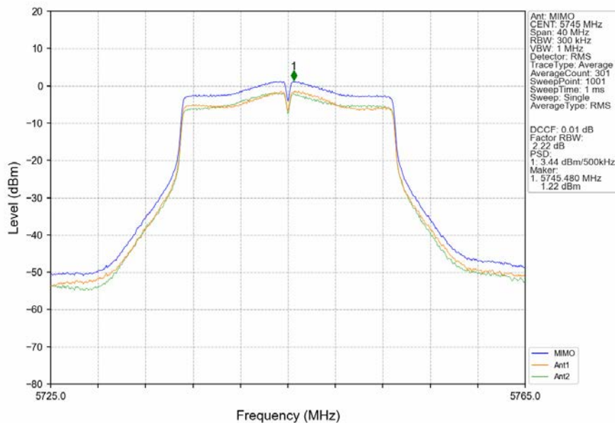
802.11ac(VHT20)_LCH_5745MHz_MIMO_NTNV
