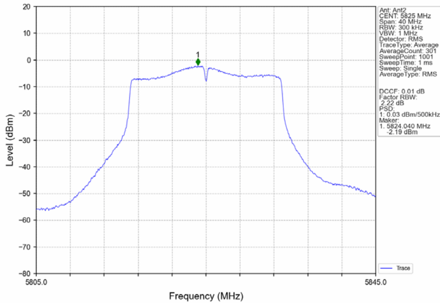
802.11ac(VHT20)_HCH_5825MHz_MIMO_NTNV
