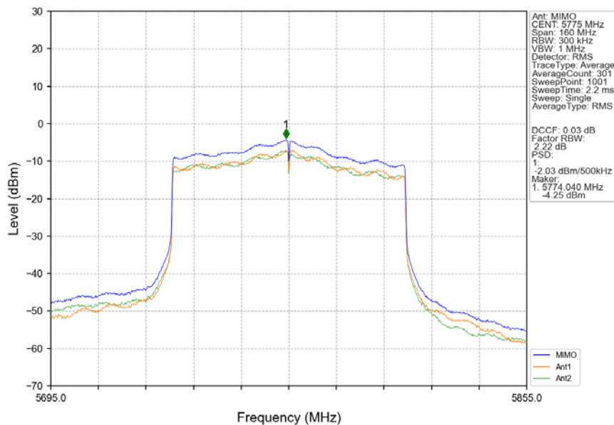
802.11ax(HEW80)_MCH_5775MHz_RU996_Left_MIMO_NTNV
