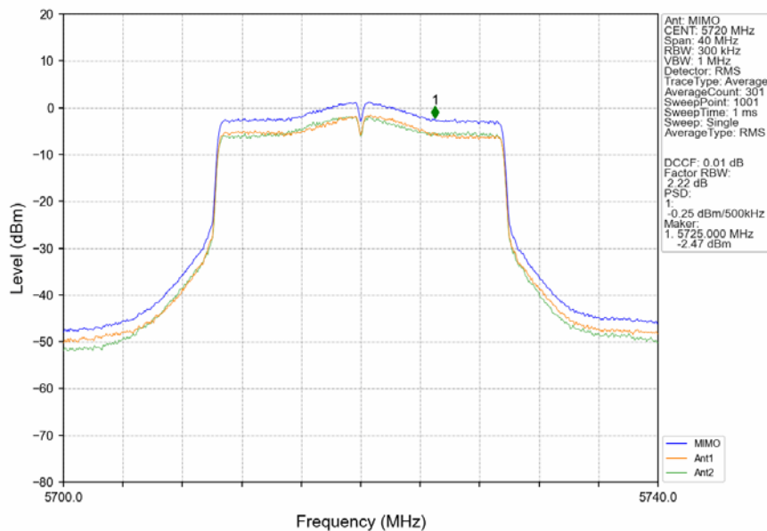
802.11ax(HEW20)_HCH_5720MHz_RU242_Left_MIMO_NTNV
