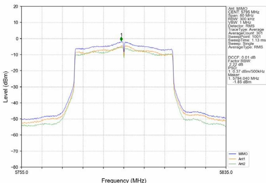
802.11ax(HEW40)_HCH_5795MHz_RU484_Left_MIMO_NTNV
