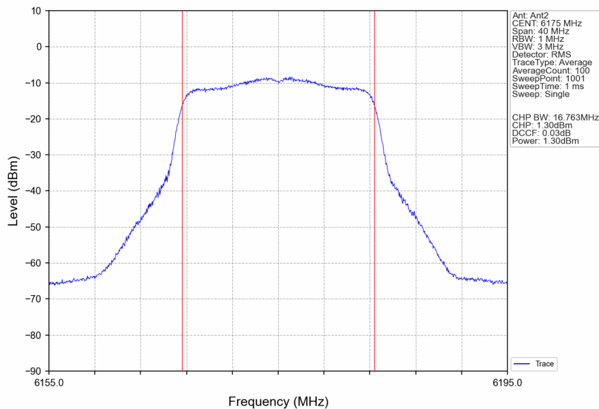
802.11a_MCH_6175MHz_Ant2_NTNV
