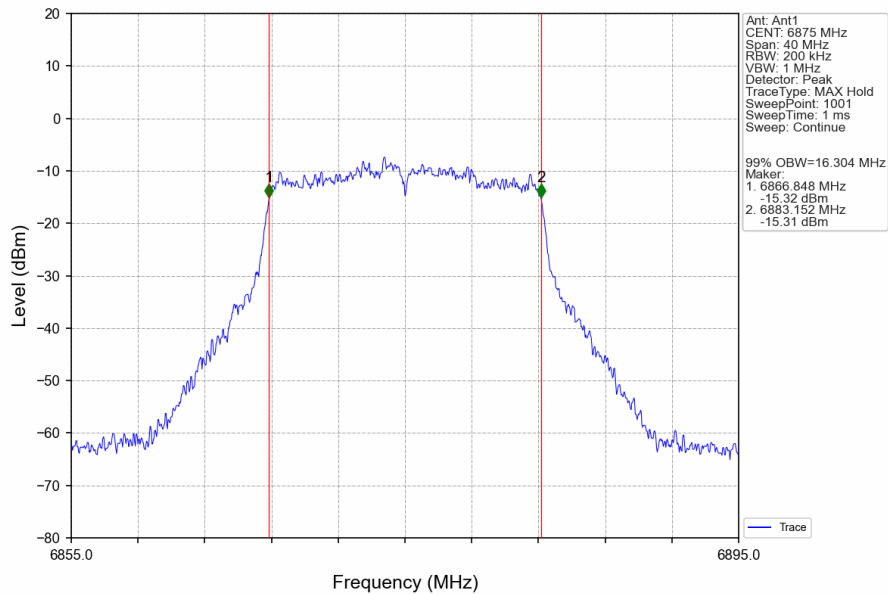
802.11ax(HEW20)_HCH_6875MHz_RU242_Left_Ant1_NTNV
