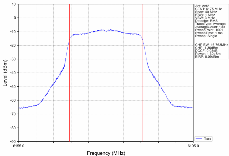
802.11a_MCH_6175MHz_Ant2_NTNV
