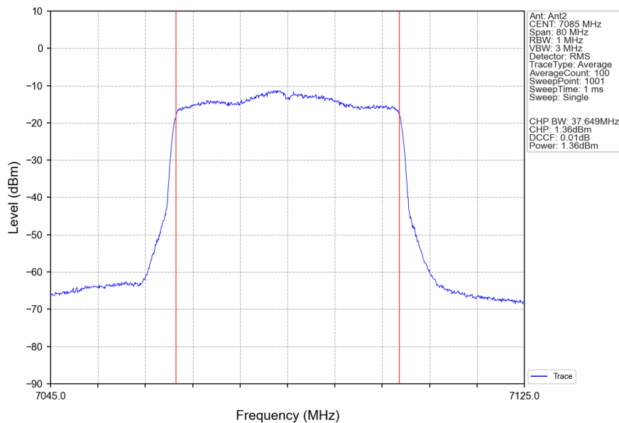
802.11ax(HEW40)_HCH_7085MHz_RU484_Left_Ant2_NTNV
