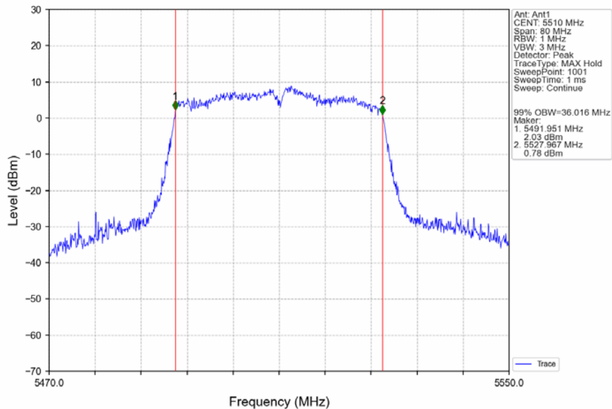
802.11ac(VHT40)_LCH_5510MHz_Ant1_NTNV
